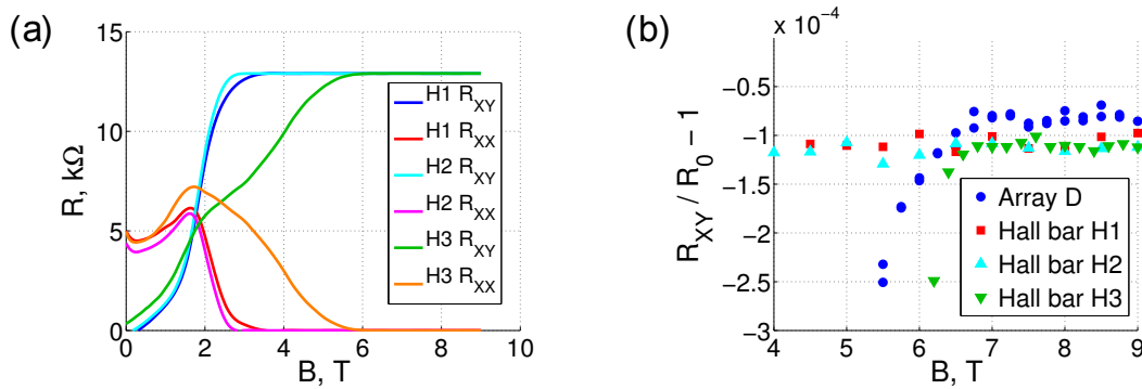
Figure 5. (a) R_{XY} and R_{XX} as a function of magnetic field in three single Hall bars: H1, H2 and H3. Measurements at negative fields were not performed since it was sufficient to achieve good quantization for one direction of the field. (b) Relative deviation of R_{XY} for the array D and three Hall bars at the strongest fields (positive fields for the Hall bars, negative fields for the array). R_0 = R_K/2 for single Hall bars and -R_K/200 for the array. The discrepancy between the single Hall bars and the array is attributed to the imprecision of the voltmeter.
