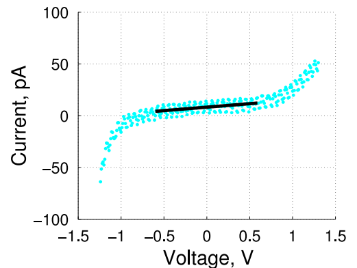
Figure 3. Measurement of the leakage current between the interconnecting wires of the quantum Hall array. The line represents a linear fit at low voltages, which gives the resistance of 150 \text{ G}\Omega .
