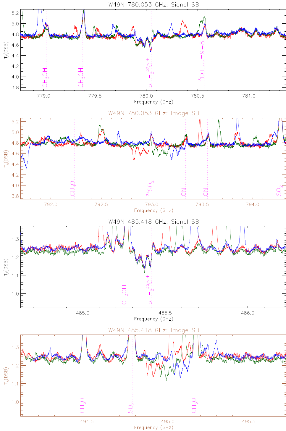
Figure 3. Same as Figure 1, except for the ortho- \text{H}_2^{37}\text{Cl}^+ 2_{12}-1_{01} (top two panels) and para- \text{H}_2^{37}\text{Cl}^+ 1_{11}-0_{00} transitions (bottom two panels) observed toward W49N.
