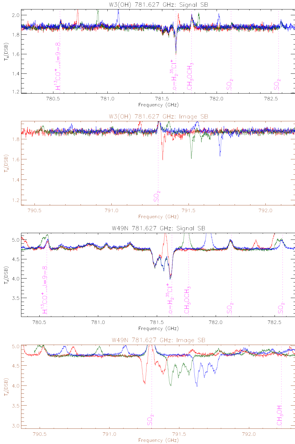
Figure 2. Same as Figure 1, except for W3(OH) (top two panels, for an assumed source velocity of -45 \text{ km s}^{-1} relative to the LSR) and W49N (bottom two panels, for an assumed source velocity of +8 \text{ km s}^{-1} relative to the LSR).
