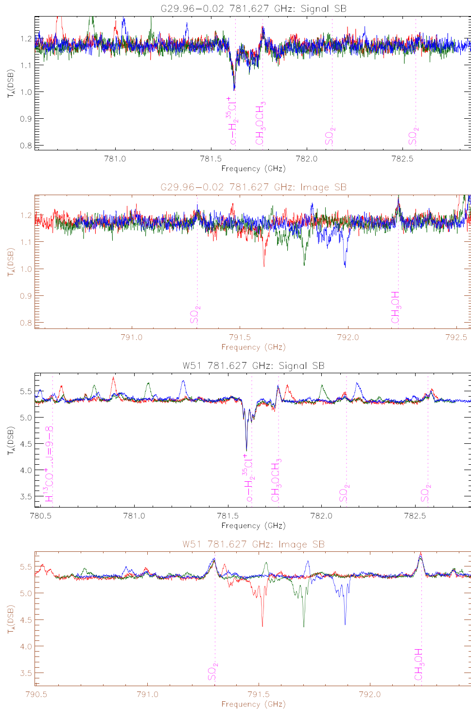
Figure 1. Spectra for 2_{12}-1_{01} transition of ortho- \text{H}_2^{35}\text{Cl}^+ obtained at three LO settings shown separately in red, green, and blue, with the frequency scale computed for either the signal or image sideband (alternate panels) in the rest frame of the source. Magenta dashed lines indicate identified spectral lines in the relevant sideband. Top two panels: G29.96-0.02, for an assumed source velocity of +98 \text{ km s}^{-1} relative to the LSR. Bottom two panels: W51, for an assumed source velocity of +55 \text{ km s}^{-1} relative to the LSR.
