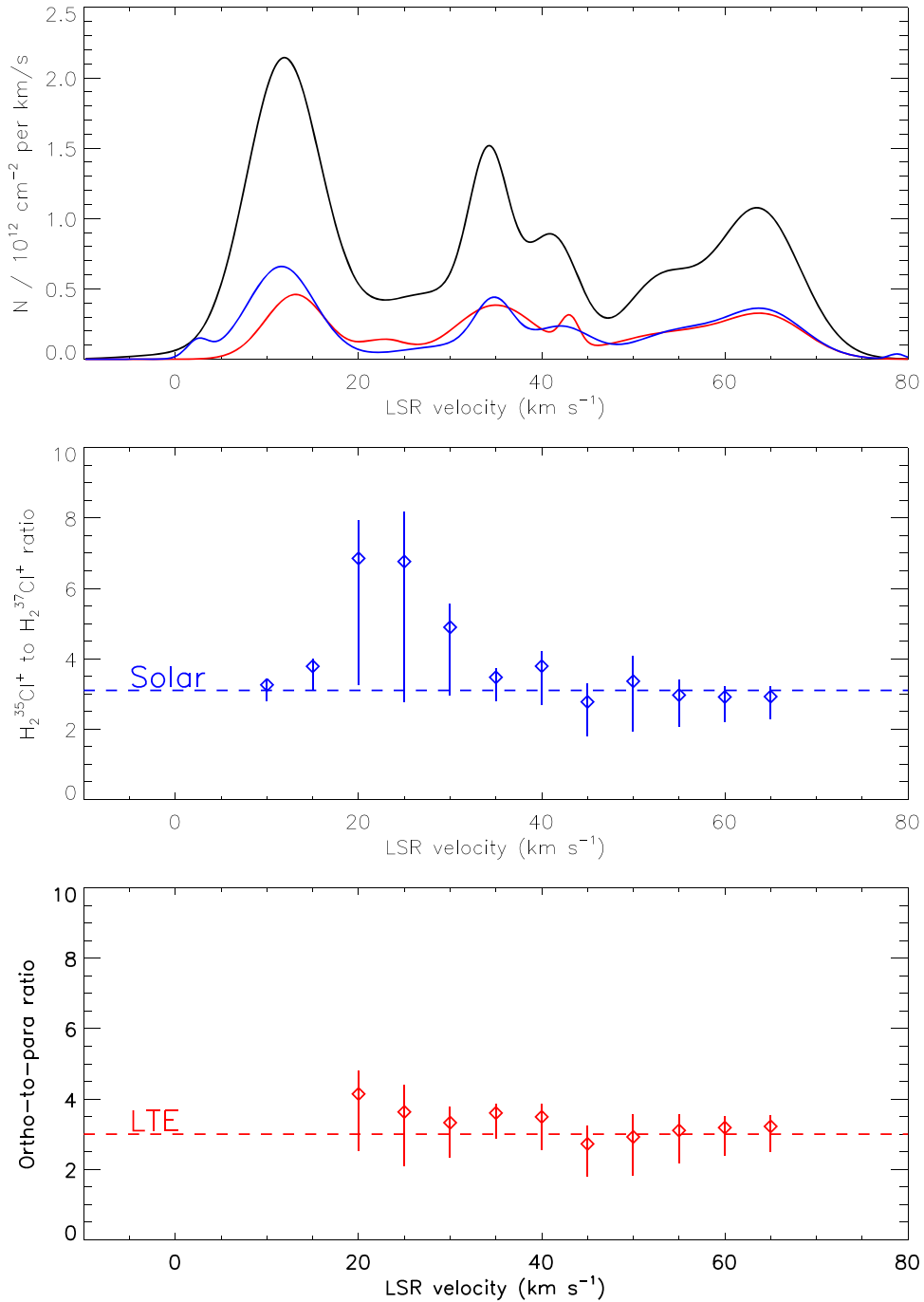
Figure 6. Top panel: derived column densities for ortho- \text{H}_2^{35}\text{Cl}^+ (black), ortho- \text{H}_2^{37}\text{Cl}^+ (blue), and para- \text{H}_2^{35}\text{Cl}^+ (red) along the sight-line to W49N. Values close the systematic velocity of the source ( 8 \text{ km s}^{-1} ) are unreliable. Middle panel: inferred ortho- \text{H}_2^{35}\text{Cl}^+ / ortho- \text{H}_2^{37}\text{Cl}^+ ratio in velocity bins of width 5 \text{ km s}^{-1} . Bottom panel: inferred ortho-to-para ratio for \text{H}_2^{35}\text{Cl}^+ in velocity bins of width 5 \text{ km s}^{-1} . Vertical error bars in the bottom two panels indicate uncertainties, and include the possibility of weak emission lines (with an assumed width of 5 \text{ km s}^{-1} and maximum antenna temperature of 50 \text{ mK} near 781 \text{ GHz} or 25 \text{ mK} near 485 \text{ GHz} ) resulting in an underestimate of the inferred optical depths.
