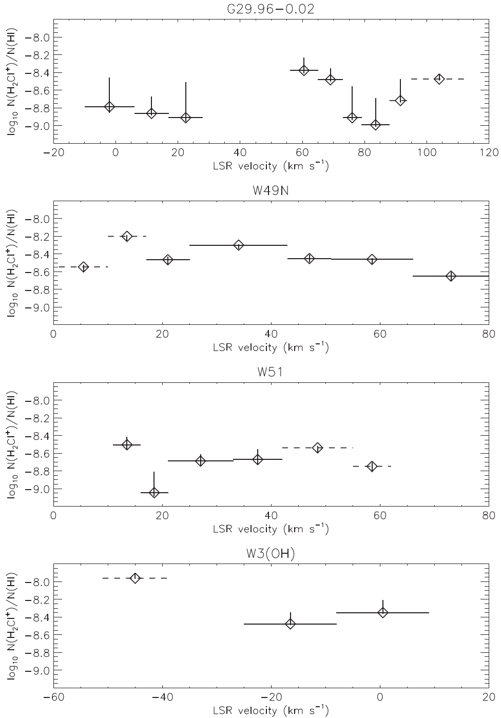
Figure 5. Inferred N(\text{H}_2\text{Cl}^+)/N(\text{H}) ratios for the velocity intervals adopted by Indriolo et al. (2015). Dashed horizontal bars indicate velocity intervals close the source systemic velocity, where the column density determinations are unreliable. Vertical error bars indicate uncertainties, and include the possibility that weak emission lines (with a width of 5 \text{ km s}^{-1} and assumed maximum antenna temperature of 50 \text{ mK} ) result in an underestimate of the inferred \text{H}_2\text{Cl}^+ optical depth.
