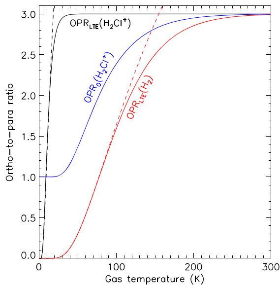
Figure 7. Ortho-to-para ratios (OPR) as a function of gas temperature. Solid black curve: \text{H}_2\text{Cl}^+ OPR in LTE. Dashed black curve: 9 \exp(-20.2 \text{ K}/T) . Solid red curve: \text{H}_2 OPR in LTE. Dashed red curve: 9 \exp(-170 \text{ K}/T) . Blue curve: initial OPR of \text{H}_2\text{Cl}^+ formed by reaction of \text{HCl}^+ with \text{H}_2 , for the scrambling mechanism (see text) and with the \text{H}_2 OPR in LTE.
