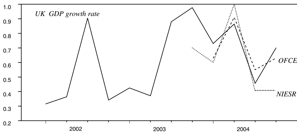
Figure 10: One-quarter-ahead forecasts of UK GDP growth rate over the last year (favourable date)
