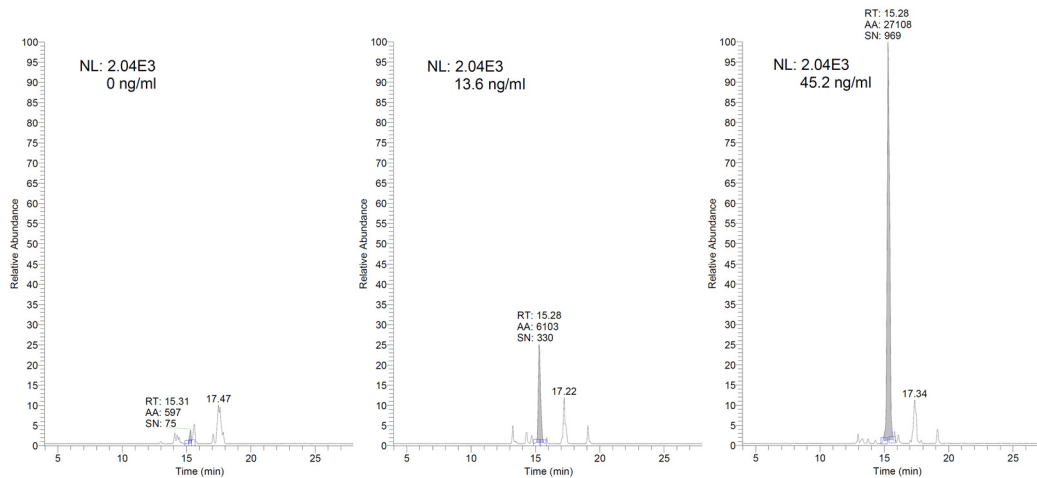
Fig 4. LC/MS chromatograms comparing different concentrations of peptide 5A in blood plasma matrix. Peptide 5A peaks in plasma matrix spiked with 0, 13.6 and 45.2 ng/mL (SRM trace: 877.7 → (412.2 + 341.1 + 946.4).
