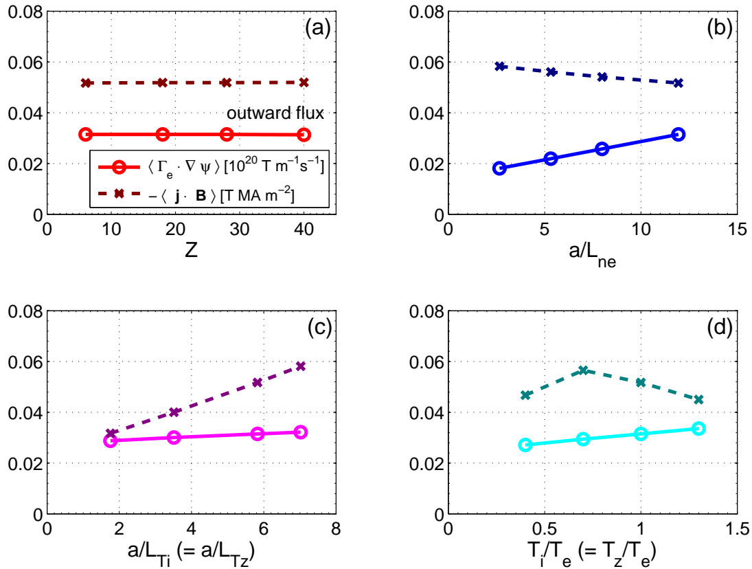
Figure 2. Main species radial flux (—○) and bootstrap current (---×) as functions of impurity charge (a), electron density gradient (b), ion temperature gradient (c), and ion temperature (d) with electron temperature fixed. Note that since \langle \Gamma_z \cdot \nabla \psi \rangle = 0 , due to ambipolarity \langle \Gamma_e \cdot \nabla \psi \rangle = \langle \Gamma_i \cdot \nabla \psi \rangle , and also that in (d) \partial T_i / \partial r (= \partial T_z / \partial r) is fixed which implies that a/L_{Ti} (= a/L_{Tz}) is varying.
