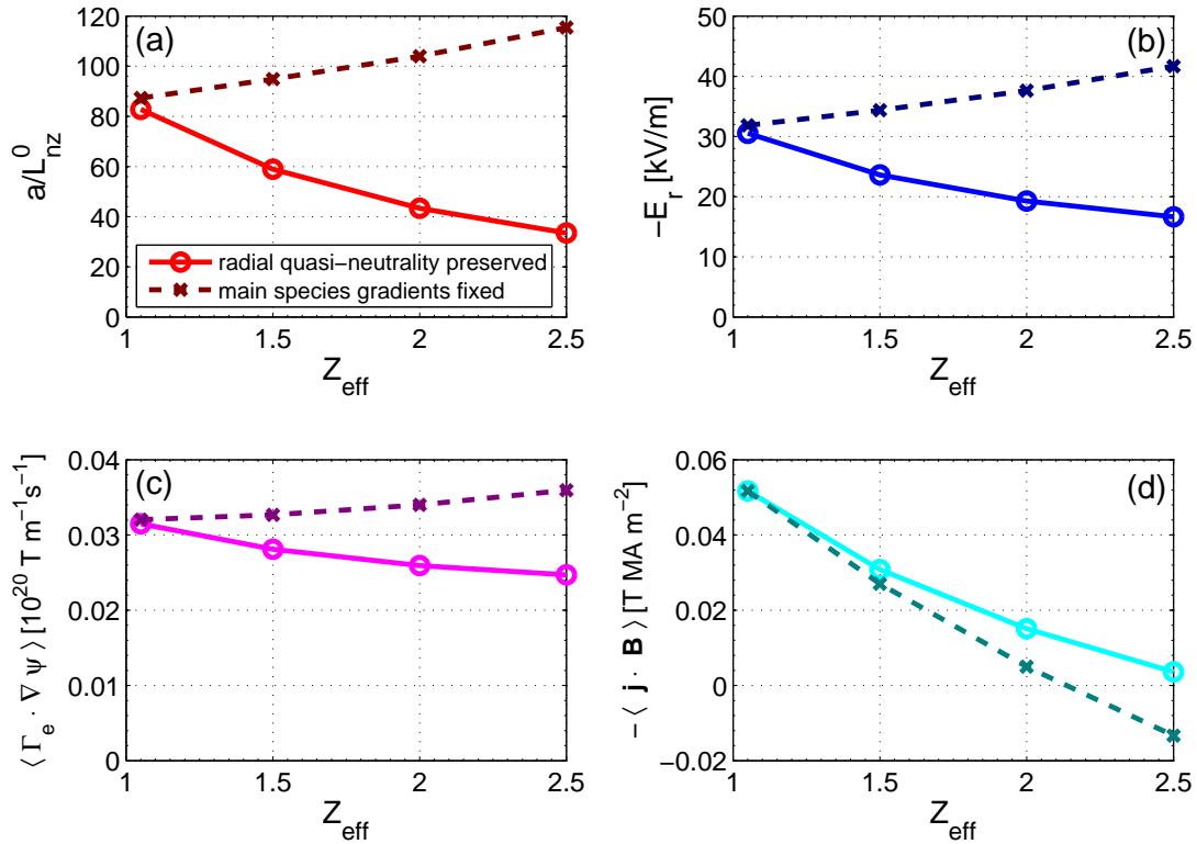
Figure 3. Impurity peaking factor (a), ambipolar radial electric field (b), main species radial flux (c), and bootstrap current (d) as functions of plasma effective charge. The analysis has been performed both maintaining radial quasi-neutrality by modifying the main ion density gradient along with the zero-flux impurity density gradient (—○), and also neglecting quasi-neutrality keeping the main species density gradients fixed (- - -×).
