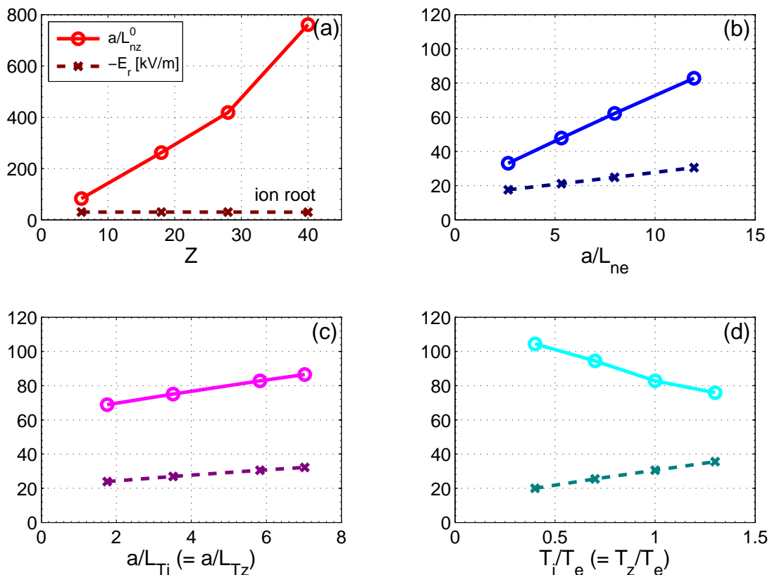
Figure 1. Impurity peaking factor (—○) and ambipolar radial electric field (---×) as functions of impurity charge (a), electron density gradient (b), ion temperature gradient (c), and ion temperature (d) with electron temperature fixed. Note that in (d) \partial T_i/\partial r ( = \partial T_z/\partial r ) is fixed which implies that a/L_{Ti} ( = a/L_{Tz} ) is varying.
