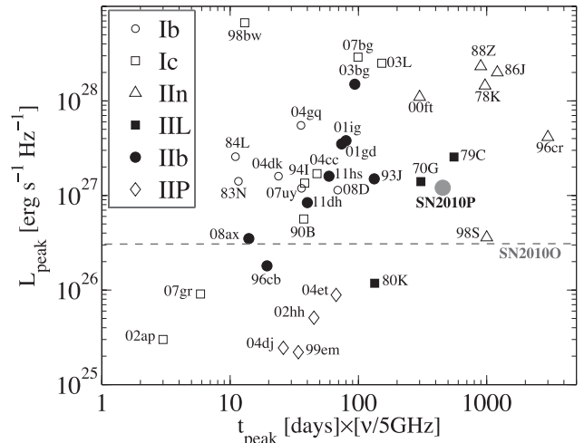
Figure 4. Peak monochromatic luminosity versus time to peak from explosion date for different types of CCSNe (hypernovae and other peculiar objects included). The first peak is used in case more than one has been reported. The dashed line represents the upper limit in luminosity for SN 2010O. References: Weiler et al. (2002) for SNe 1970G, 1979C, 1980K, 1983N, 1984L, 1986J, 1988Z, 1990B and 1994I; Pooley et al. (2002) for 1998S and 1999em; Wellons, Soderberg & Chevalier (2012) for 2004cc, 2004dk and 2004gq; van der Horst et al. (2011) for 2007uy and 2008D; Schlegel et al. (1999) for 1978K; Weiler et al. (2007) for 1993J; Weiler et al. (1998) for 1996cb; Bauer et al. (2008) for 1996cr; Weiler, Panagia & Montes (2001) for 1998bw; Pérez-Torres et al. (2009a) for 2000ft; Stockdale et al. (2007) for 2001gd; Ryder et al. (2004) for 2001ig; Berger, Kulkarni & Chevalier (2002) for 2002ap; Chevalier, Fransson & Nymark (2006) for 2002hh; Soderberg et al. (2005) for 2003L; Soderberg et al. (2006) for 2003bg; Beswick et al. (2005) for 2004dj; Martí-Vidal et al. (2007) for 2004et; Salas et al. (2013) for 2007bg; Soderberg et al. (2010) for 2007gr; Roming et al. (2009) for 2008ax; Maeda (2012) for 2011dh (see also Horesh et al. 2013); Bufano et al. (2014) for 2011hs.
