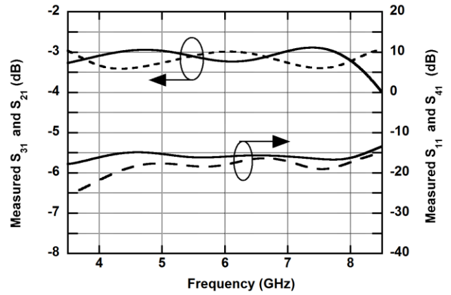
Fig. 9: Measured performance (through, coupled, return loss and isolation) of the hybrid assembly.
