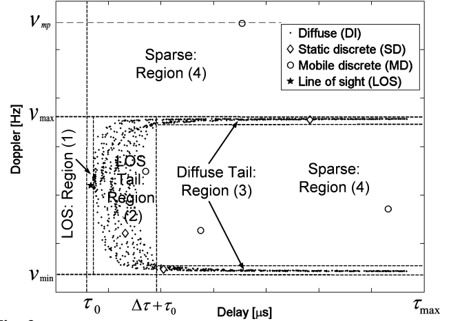
Fig. 2: Delay-Doppler domain representation of V2V channel. Delay-Doppler spreading function is confined in a U-shape area.
