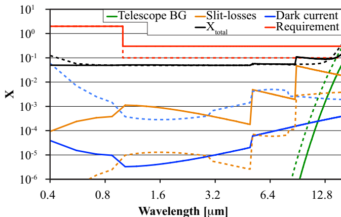
Fig. 8. Photometric stability performance expressed as X -factor for the brightest (solid line) and the faintest sources (dashed line). The individual contributions from the telescope thermal background, slit-losses and dark current are shown. System noise components with constant X -values are not shown (see Table 3). The required values for X are plotted in solid red, the goal values are plotted in dashed red.
