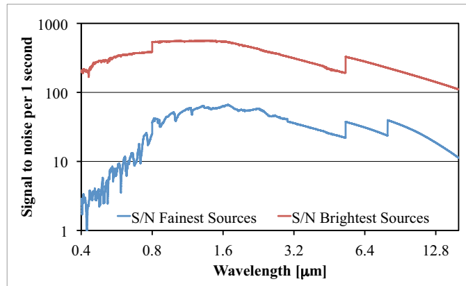
Fig. 7. S/N for 1 second integration time for the brightest stars (K0V, K_{\text{mag}} = 4.0 , red line) and faintest stars (for \lambda < 3 \mu\text{m} : M5V, K_{\text{mag}} = 8.8 , for 3 \mu\text{m} \leq \lambda \leq 8 \mu\text{m} : G0V, K_{\text{mag}} = 9.0 , and for \lambda > 8 \mu\text{m} : G0V, K_{\text{mag}} = 8.8 , blue line).
