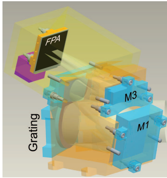
Fig. 4. Three mirror anastigmats camera with grating and detector of channel IR1. The camera housing is indicated in half-transparency.
