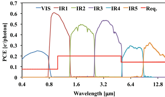
Fig. 6. Photon conversion efficiency of the instrument compared with the mission requirement (red line).
