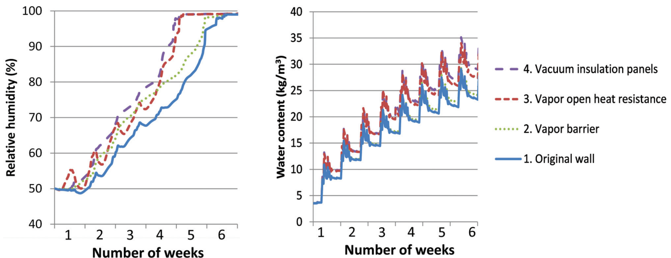
Figure 9 Simulation of the relative humidity 60 \text{ mm} ( 2.4 \text{ in.} ) from the interior surface and the total water content in the 250 \text{ mm} ( 9.8 \text{ in.} ) wall composed of homogenous historical bricks and fine lime cement mortar between the bricks with varying interior boundary conditions during the climate cycle defined in Table 2.
