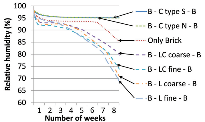
Figure 8 Relative humidity in the middle of the mortar in a 250 mm (9.8 in.) extruded brick (B) wall with varying mortar properties placed indoors in Trondheim, Norway, starting on October 1 based on data from the WUFI database (Fraunhofer IBP 2010). For comparison, a wall with only brick is simulated under the same conditions.
