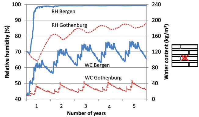
Figure 5 Relative humidity in the middle of a 380 mm (15 in.) thick homogenous brick wall (marked by a cross with circle in the right figure) and total water content in the wall, which is made of extruded brick and coarse lime cement mortar. The wall is facing south in both Bergen and Gothenburg with a 0.3 rainwater absorption factor.
