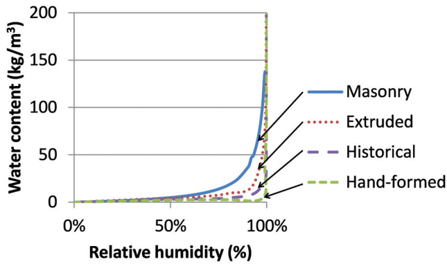
Figure 4 Sorption isotherms at 23°C of the four types of brick included in the study based on data from WUFI 2D (Fraunhofer IBP 2010).
