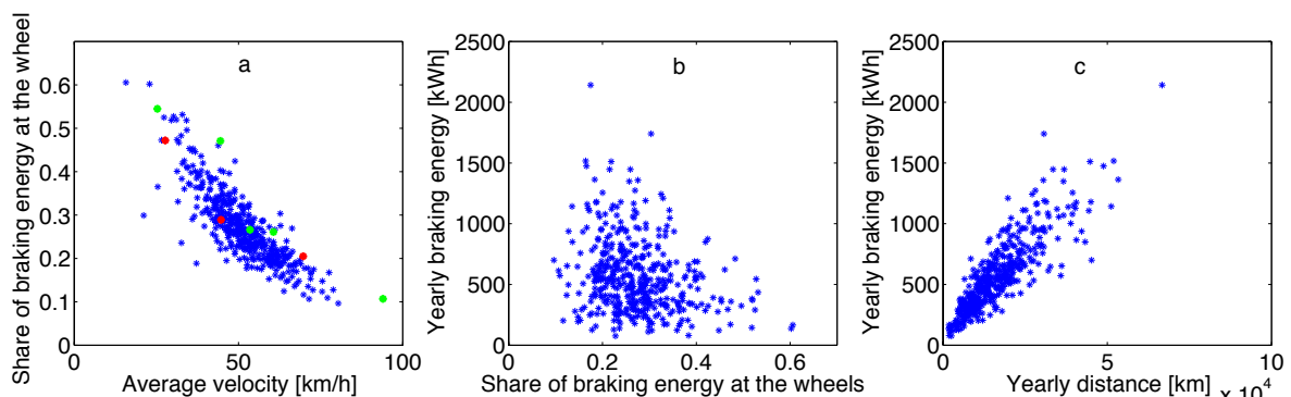
Figure 3. For the assumed car, for each movement pattern, a) the share of energy (at the wheels) lost through braking as a function of average velocity, red dots represents the values for NEDC, ECE and EUDC and green dots represents WLTP, low, middle, high, extra high; b) the total energy lost yearly (at the wheels) through braking as a function of the share of energy (at the wheels) lost through braking; c) total energy lost yearly (at the wheels) through braking as a function of the yearly mileage.
