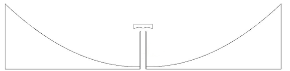
Fig. 6. G2DMULT geometry for the cross section of the 1D reflector (E-plane)
