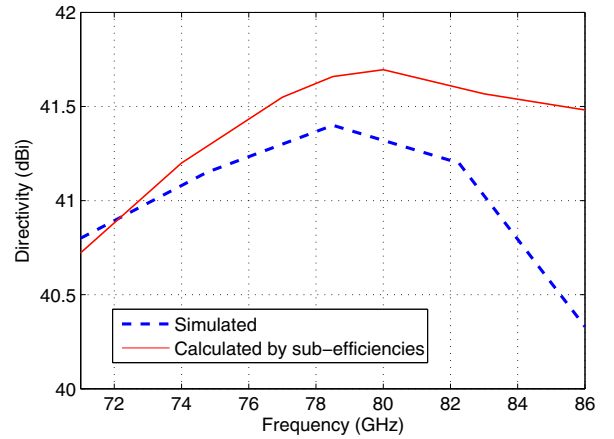
Fig. 10. Directivity over the E-band obtained by two methods: 1) simulation; 2) D = D_{max} - e_{sp} - e_{\phi} - e_b - e_{ill} , where e_{sp} is the spillover loss, e_{\phi} the phase loss, e_b the blockage loss and e_{ill} the illumination loss.
