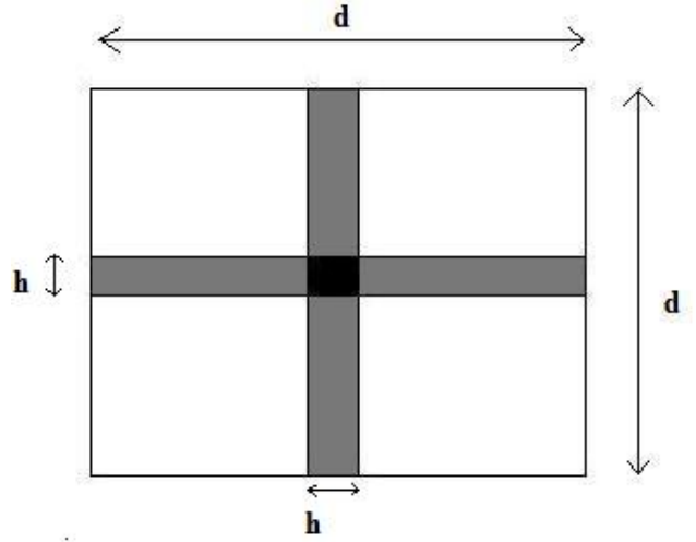
Fig. 2. Blockage in the rectangular aperture of the cylindrical reflector (a is the total area of the aperture, b is the area that is blocked along the two dimensions and corresponds to the grey area of the figure and c is the black common blocked area at the center)
