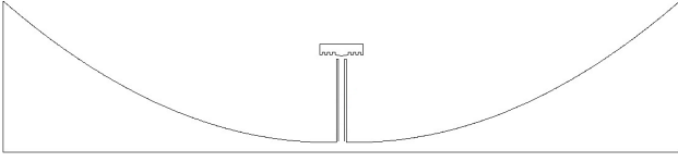
Fig. 7. G2DMULT geometry for the cross section of the cylindrical reflector (H-plane)
