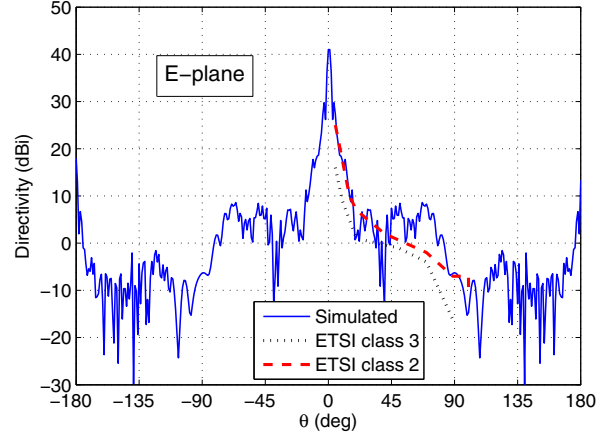
Fig. 4. Calculated E-plane of the cylindrical reflector for f = 78.5 GHz
