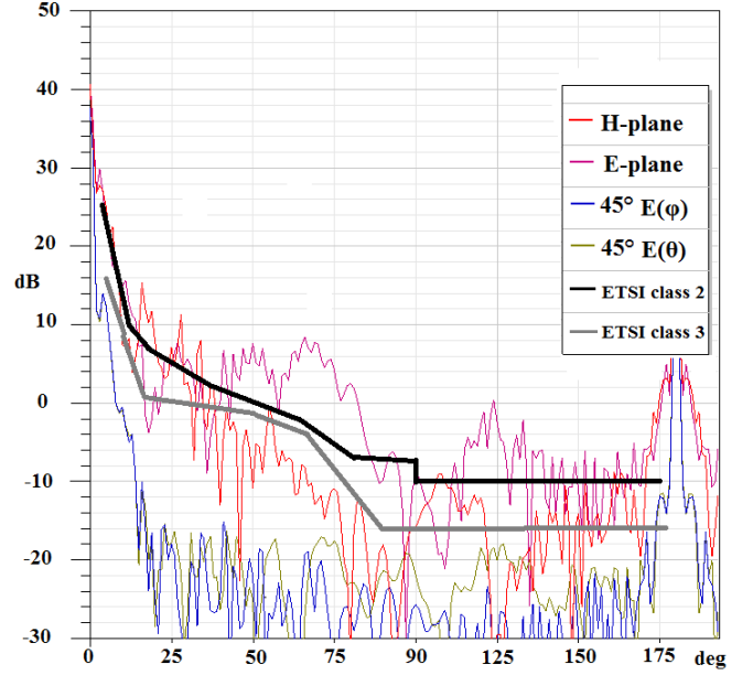
Fig. 9. Simulated E, H and 45°-plane of cylindrical reflector for f = 78.5 GHz
