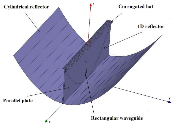
Fig. 1. Cylindrical parabolic reflector antenna
