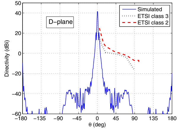
Fig. 5. Calculated 45°-plane of the cylindrical reflector for f = 78.5 GHz
