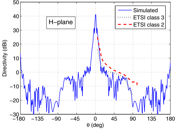
Fig. 3. Calculated H-plane of the cylindrical reflector for f = 78.5 GHz
