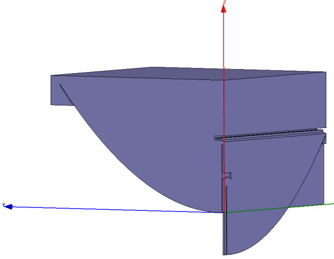
Fig. 8. One quarter of the cylindrical reflector as simulated in HFSS
