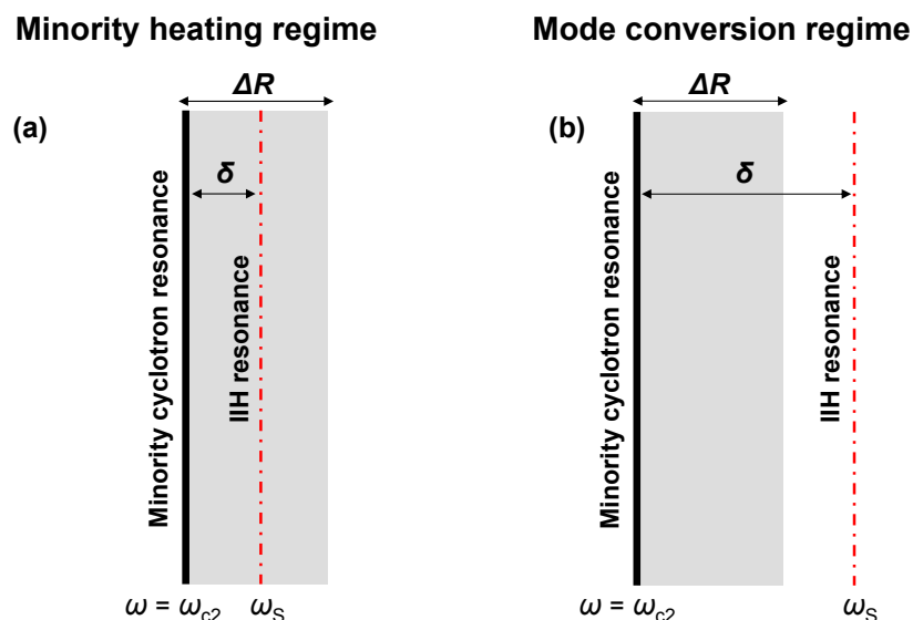
Figure 4. Transition from MH (a) to MC (b) heating regime occurs when the IIIH resonance passes through the Doppler broadened minority cyclotron layer (the scheme corresponds to the inverted ICRH scenario, for which the IIIH resonance is to the LFS of the minority IC layer).
