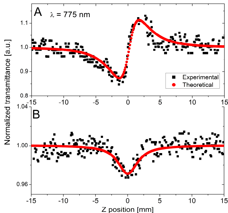
Fig.1. Representative CA (A) and OA (B) Z-scan traces and the theoretical fits for EB-dimer at 775 nm (1 % solution in DMSO). The CA trace was divided by the OA trace to obtain a purely refractive effect.
