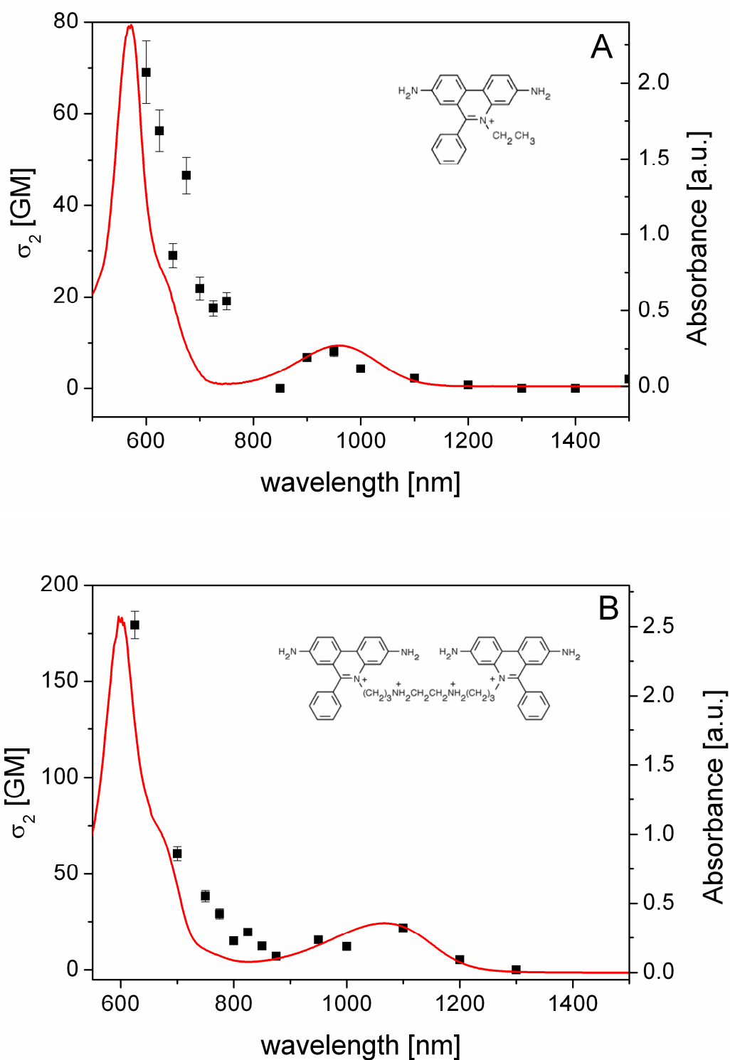
Fig.2. 1PA (red line) and 2PA (black squares) spectra of EB (A) and EB-dimer (B). One photon spectrum is plotted with the wavelength multiplied by a factor of two. Inset shows the EB and EB-dimer molecular structure.
