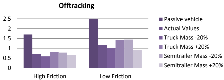
Figure 5.7 Effect of vehicle mass uncertainties on the achieved offtracking
