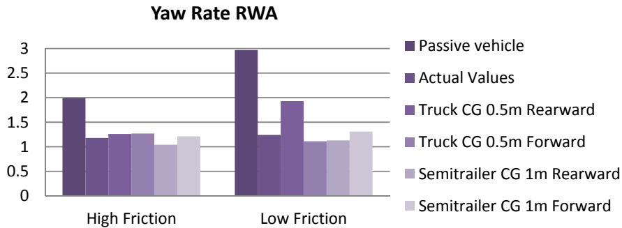
Figure 5.10 Effect of CG location uncertainties on the achieved yaw rate RWA
