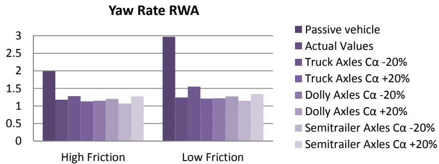
Figure 5.4 Effect of tire cornering stiffness ( C\alpha ) uncertainties on the achieved yaw rate RWA
