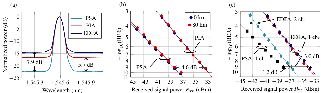
Figure 2: a) Signal spectra out from the pre-amplifiers under test. The spectra (0.1nm resolution) are normalized to their peak values to better compare noise floor levels. b) BER curves comparing FOPA performance with a lumped loss (0km) or fiber link (80km) between copier and PSA. The legend indicates link length used. c) BER curves comparing PSA system performance against the EDFA-based systems. The red and blue EDFA single channel curves correspond to single channel detection of the 1543 and 1545nm wavelengths respectively
