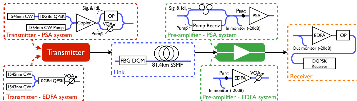
Figure 1: Set-up for both EDFA and FOPA pre-amplifier characterization. OP: Optical processor, VOA: Variable optical attenuator, PC: Polarization controller, FBG DCM: Fiber Bragg grating dispersion compensation module, P REC : Received power measurement point in BER tests.
