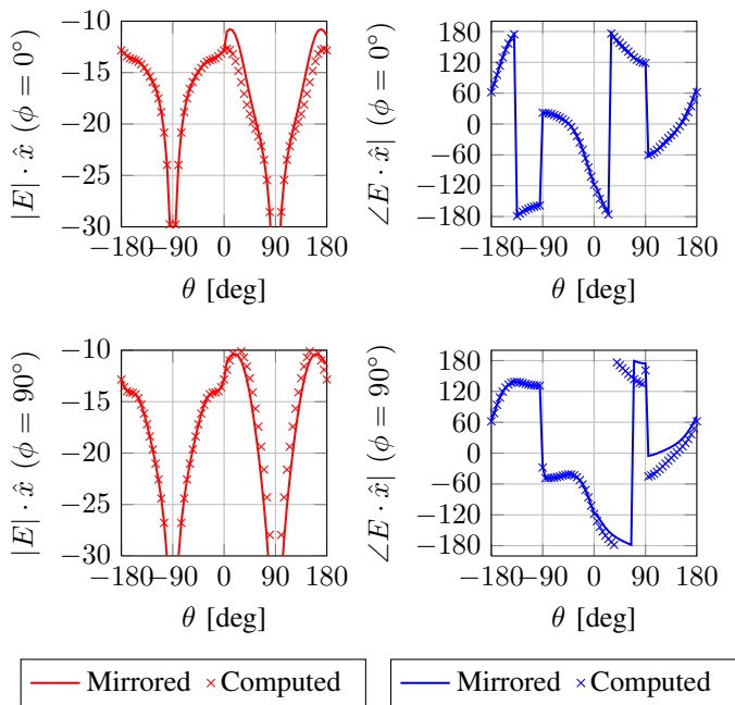
Fig. 7. Comparisons between mirrored and directly computed beam pattern cuts for port 4 of four folded dipoles arranged in an identical port layout as shown in Fig. 4, simulated at 5 GHz
