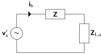
Fig. 2. Equivalent voltage excitation for case “a” to realise current \mathbf{i}_b in situation “b”.
