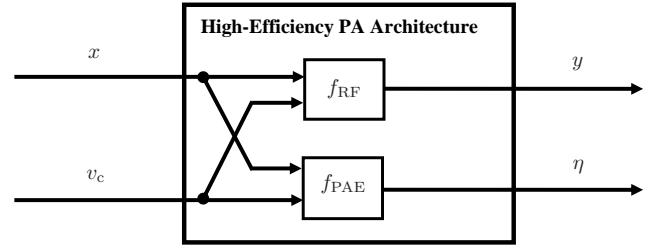
Fig. 2. A general model for high-efficiency power amplifier architectures. x is the RF input signal, v_c is the envelope signal, y is the output RF signal, \eta is the instantaneous power-added efficiency, f_{RF} and f_{PAE} are transfer functions representing the RF path and output PAE path, respectively.
