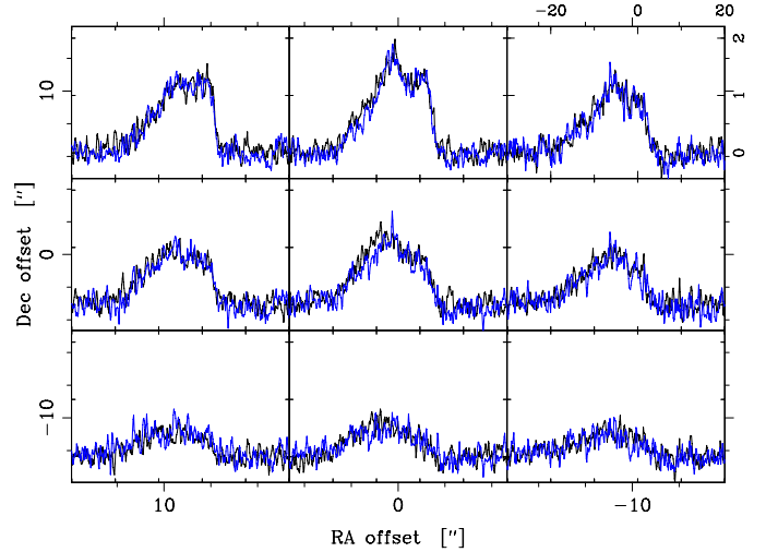
Fig. B.1. CO(10–9) spectra toward HH 54. The black spectra are from the HIFI observation 1342180798, while the blue spectra are from the observation 1342190901. The horizontal and vertical polarisations have been averaged together (see text).
