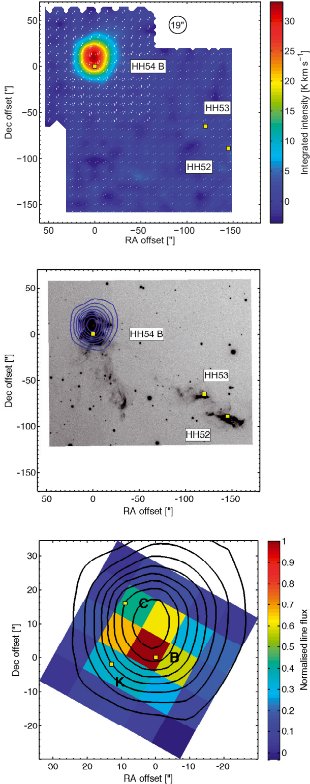
Fig. 1. Upper panel: false colour map of the CO(10–9) integrated intensity in the blue line wing (from +2.4 \text{ km s}^{-1} to -30 \text{ km s}^{-1} ). The positions of HH 54 B, HH 53, and HH 52 are indicated with yellow squares. The readout positions for the on-the-fly and raster maps are indicated with white dots. Middle panel: CO(10–9) map of the integrated intensity obtained with HIFI in the blue line wing overlaid on an H\alpha image from Caratti o Garatti et al. (2009). Contours are from 5.5 to 33.6 \text{ K km s}^{-1} in steps of 3.5 \text{ K km s}^{-1} . Lower panel: a zoom of the CO(10–9) integrated intensity overlaid on the \text{H}_2\text{O}(2_{12}-1_{01}) emission obtained with PACS. The positions of HH 54 B, C and K as indicated in Giannini et al. (2006) are indicated with yellow squares.
