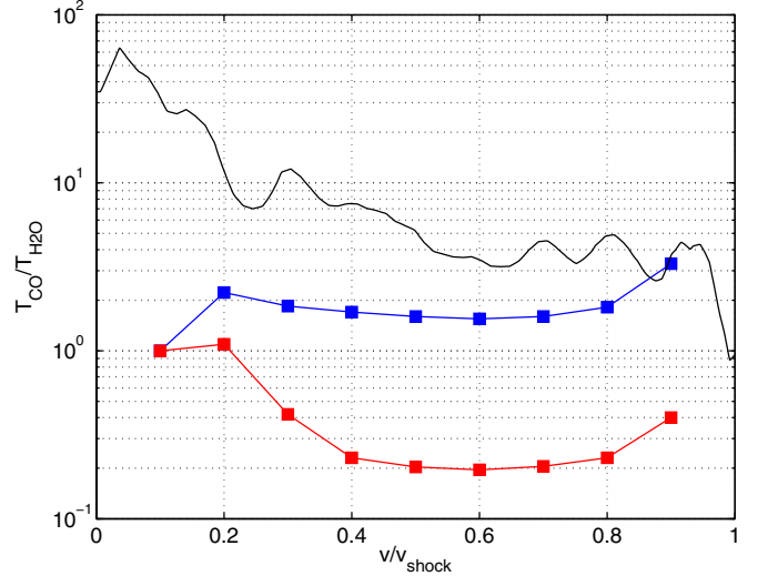
Fig. 15. Line ratios between CO (5–4) and H 2 O (1 10 –1 01 ). The ratio as measured from Odin is indicated with a black line. The predictions presented by Flower & Pineau des Forêts (2010) for v_{\text{shock}} = 20 km s -1 are plotted in blue for n_{\text{H}} = 2 \times 10^4 cm -3 and in red for n_{\text{H}} = 2 \times 10^5 cm -3 .
