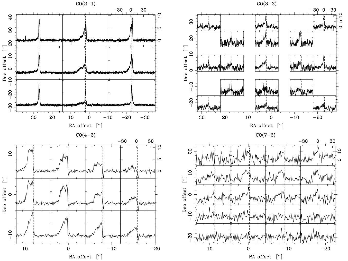
Fig. 4. Same as Fig. 3, but for the CO (2–1), CO (3–2), CO (4–3), and CO (7–6) maps obtained with SEST and APEX. The APEX maps have been regrided with a map spacing equal to 8'' for CO (4–3) and 9'' for CO (7–6). Note that the CO (4–3) spectra may be contaminated with OFF beam contribution.
