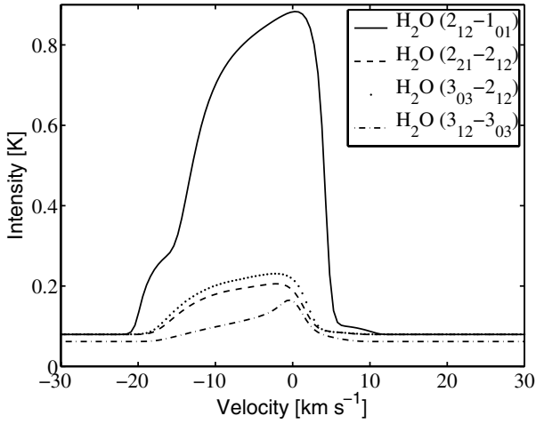
Fig. 12. Line profile predictions for the \text{H}_2\text{O}(2_{12}-1_{01}) , \text{H}_2\text{O}(2_{21}-2_{12}) , \text{H}_2\text{O}(3_{03}-2_{12}) , and \text{H}_2\text{O}(3_{12}-3_{03}) spectra as observed with HIFI.
