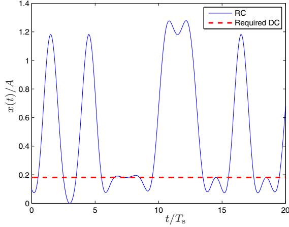
Fig. 2: The normalized transmitted signal x(t)/A using an RC pulse (7) with \alpha = 0.6 as q(t) . It can be seen that without using the bias \mu = 0.184 , the raised-cosine pulse would create a signal x(t) that can be negative.
