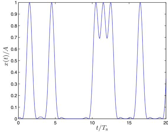
Fig. 3: The normalized transmitted signal x(t)/A using an SRC pulse (11) with \alpha = 0.6 as q(t) . In this case, the required DC \mu is zero.
