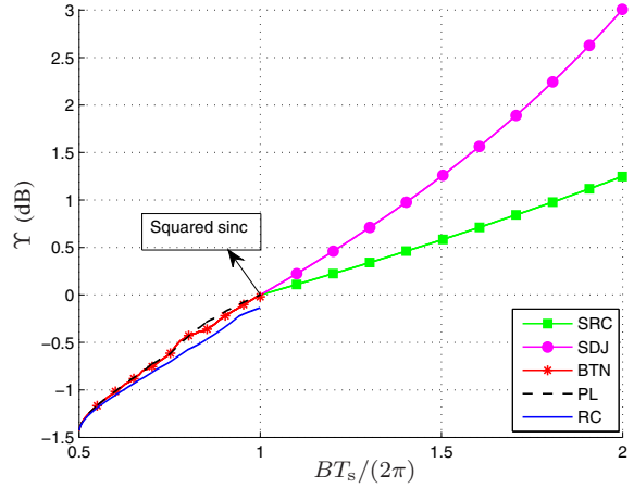
Fig. 5: The optical power gain \Upsilon versus normalized bandwidth BT_s/(2\pi) . The electrical power of noiseless samples for all pulses is equal. The results for BT_s < 2\pi are novel, while those for BT_s \geq 2\pi are prior knowledge.
