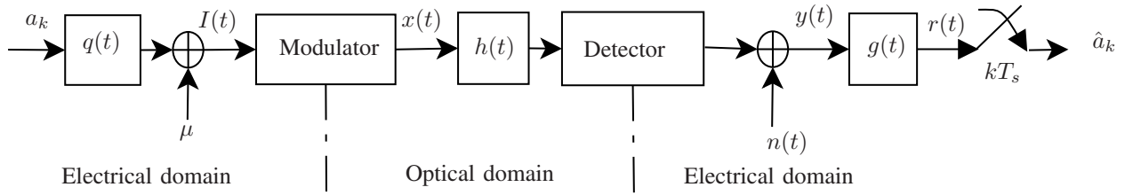
Fig. 1: Baseband system model, where a_k is the k -th input bit, q(t) is an arbitrary pulse, \mu is the DC bias, I(t) is the transmitted electrical signal, x(t) is the optical intensity, h(t) is the channel impulse response, n(t) is the noise, g(t) is the impulse response of the receiver filter, and \hat{a}_k is an estimate of a_k .
