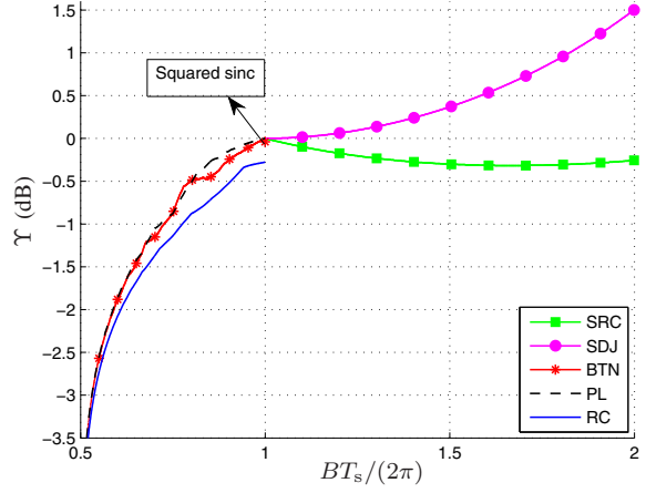
Fig. 6: The optical power gain versus normalized bandwidth BT_s/(2\pi) . The BER for all pulses is equal.
