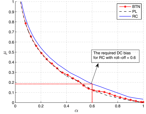
Fig. 4: The minimum DC bias \mu vs. roll-off factor \alpha for all pulses discussed in Sec. III-A.
