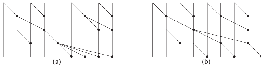
Fig. 20. (a) LF_0 , the minimum depth Ladner–Fischer network, for nine inputs; it has 13 operators and depth 4 (b) A smaller 9-input network (with 12 operators, depth 4) made from LF_18 , and one further operator to take care of the last input. This network is DSO. This illustrates the fact that LF_0 does not always give optimal networks.
