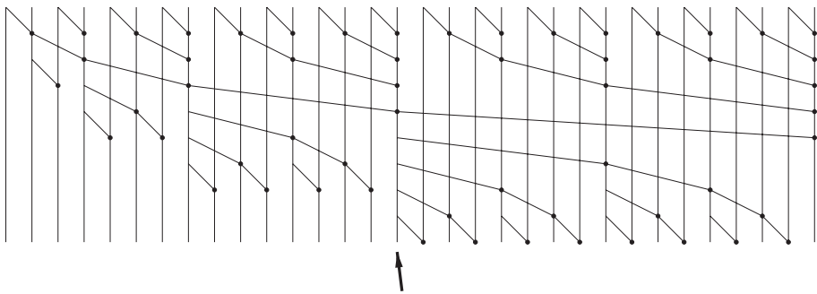
Fig. 6. The Brent–Kung construction, fanout 2, 32 inputs, depth 9, 57 operators. The arrow below the diagram points to a line that has (from top to bottom) first four combining nodes and then four duplicating nodes. The output of the bottom-most combining node on that line is fanned out to a total of six different destinations, but this fanout occurs at successive levels, so that the overall fanout of the network is only 2.
