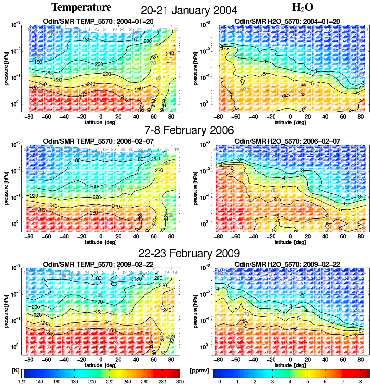
Figure 3. Pressure (2 hPa to 0.001 hPa) versus latitude cross sections of (left) zonal-mean mesospheric temperature and (right) water vapor mixing ratio on (top row) 20–21 January 2004, 7–8 February 2006, and (bottom row) 22–23 February 2009. Dot-dashed lines are approximate altitudes in kilometer.
