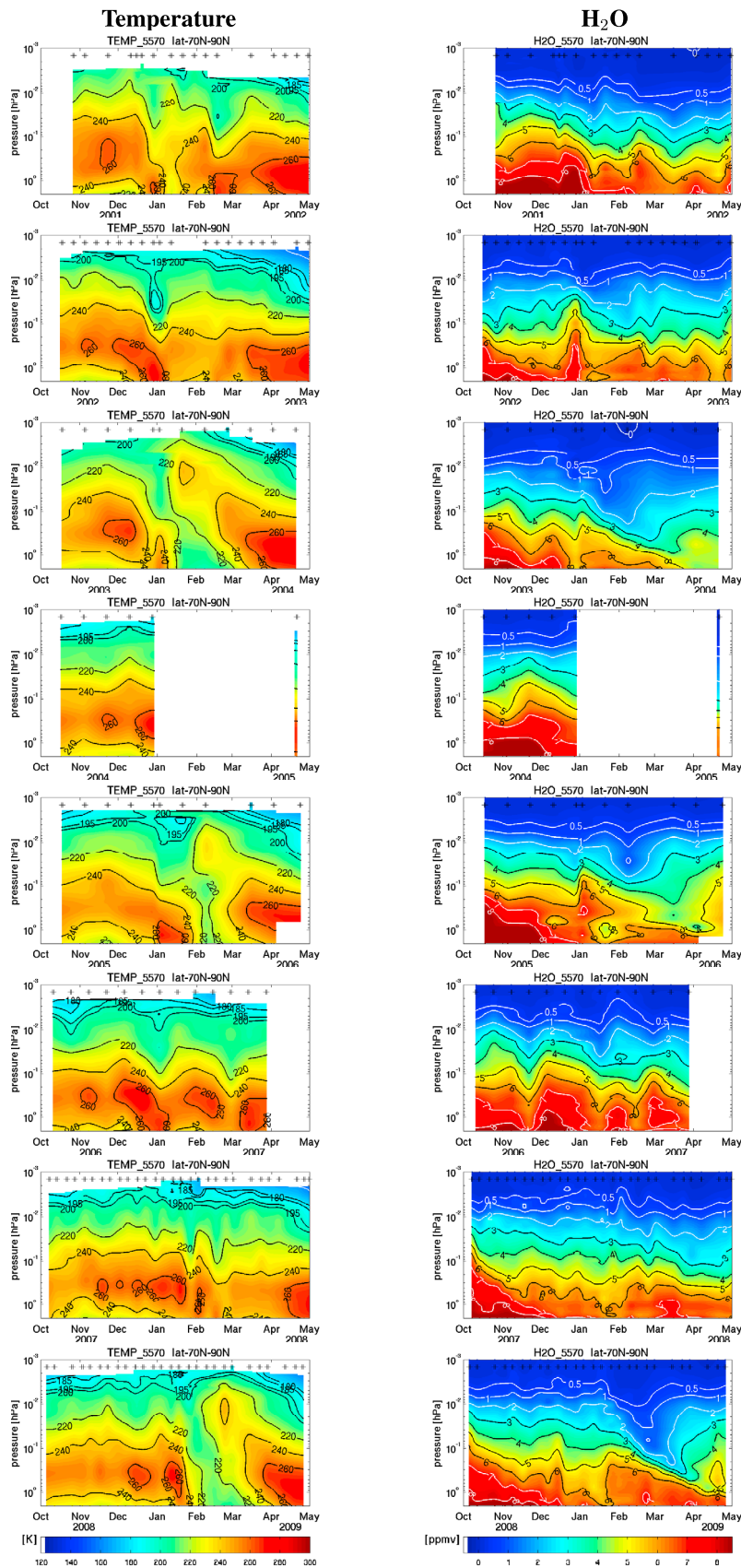
Figure 4. Pressure (2 hPa to 0.001 hPa) versus time (October–April) cross sections of zonal-mean mesospheric temperature (left) and water vapor mixing ratio (right) in the NH high latitudes (poleward of 70°N) through 8 winters measured by Odin/SMR (2001–2002 through and 2008–2009).
