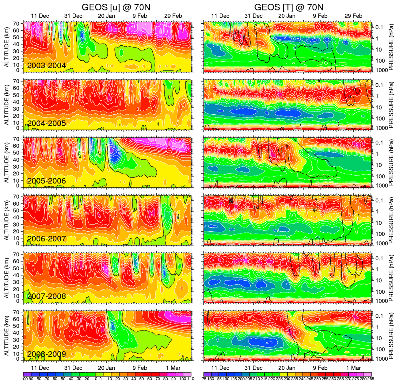
Figure 5. Altitude-time cross section of zonal-mean zonal wind (left) and temperature (right) from NASA GEOS-5 analyses at 70°N, from ground up to 70 km, from December to March for winters 2003–2004 to 2008–2009.
