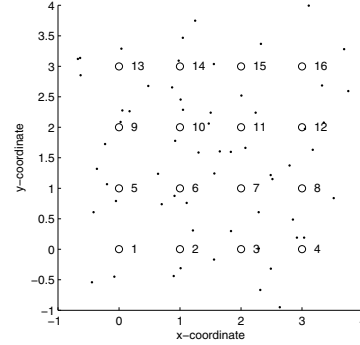
Fig. 3. An example of the simulated network of 16 clusters with sinks (circles) and nodes (dots).
