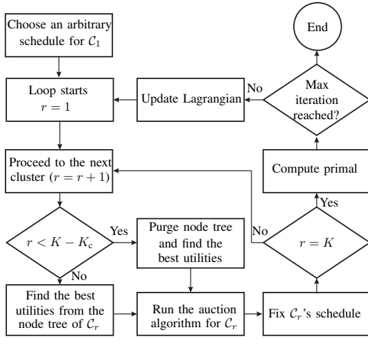
Fig. 2. The flowchart of the simplified scheduling algorithm.
