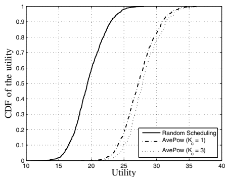
Fig. 5. The CDF of utility for AvePow method and for K_c = 1 and 3 versus random scheduling utility.
