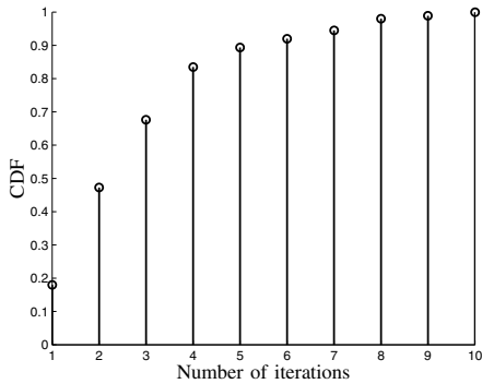
Fig. 4. The cumulative distribution function (CDF) of the iteration number for which the best performing schedule is found.
