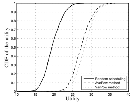
Fig. 6. The CDF of utility for AvePow versus VarPow for K_c = 1 .
