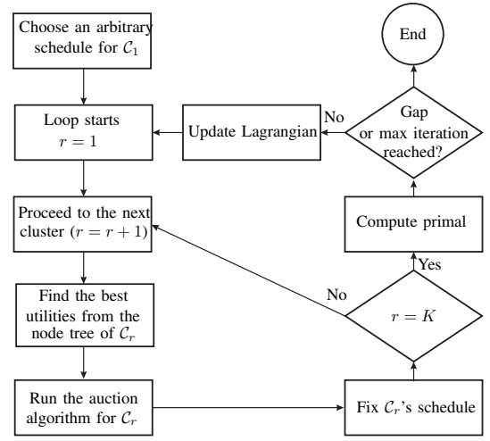
Fig. 1. The flowchart of the algorithm in [8].
