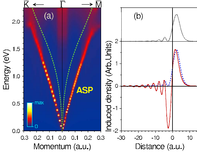
FIG. 4. (Color online) (a) 2D plot of \text{Im}[g(\mathbf{q}_{\parallel}, E)] along the \overline{\Gamma K} (to the left) and \overline{\Gamma M} (to the right) directions. Bright spots show the ASP dispersion and thin dotted line presents dispersion of a 2D plasmon for an unsupported K-derived QWS. (b) Upper panel gives the QWS charge density distribution, n_{\text{QWS}} , in the direction perpendicular to the surface. Lower panel shows induced charge density corresponding to the ASP, \rho_{\text{ASP}}^{\text{ind}} , (solid line) and the one obtained taking only QWS into account in calculation of the response function, \rho_{\text{2D}}^{\text{ind}} , (dashed line) at q_{\parallel}=0.0569 a.u. -1 . One can see how \rho_{\text{2D}}^{\text{ind}} follows closely to n_{\text{QWS}} , while \rho_{\text{ASP}}^{\text{ind}} displays a pronounced oscillatory behavior, mixing with the Be substrate. The K monolayer (Be crystal) is located at z=0 (negative z ).
