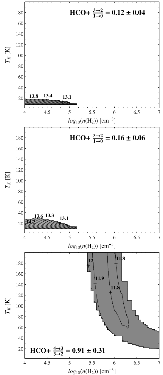
Fig. B.2. Top - Excitation conditions modeled for the \frac{3-2}{1-0} line ratio of \text{HCO}^+ , when considering the estimated starburst contribution factor f_{\text{SB}} = 0.45 , but a larger source size \theta_S = 2'' . Middle - Excitation conditions modeled for the \frac{3-2}{1-0} line ratio of \text{HCO}^+ , when considering a larger starburst contribution factor f_{\text{SB}} = 0.60 , and the common source size \theta_S = 1.5'' . Bottom - Excitation conditions modeled for the \frac{4-3}{3-2} line ratio of \text{HCO}^+ , when reducing the \text{HCO}^+ J=4-3 line intensity by a factor 1.5. The higher transition J=4-3 still traces mostly the dense and warm gas ( n(\text{H}_2) \geq 10^{5.4} \text{ cm}^{-3} , T_K \geq 20 K), whereas the \frac{3-2}{1-0} line ratio indicates that those lines would trace less dense ( n(\text{H}_2) < 10^{5.2} \text{ cm}^{-3} ) and cold ( 10 \text{ K} < T_K < 30 K) gas.
