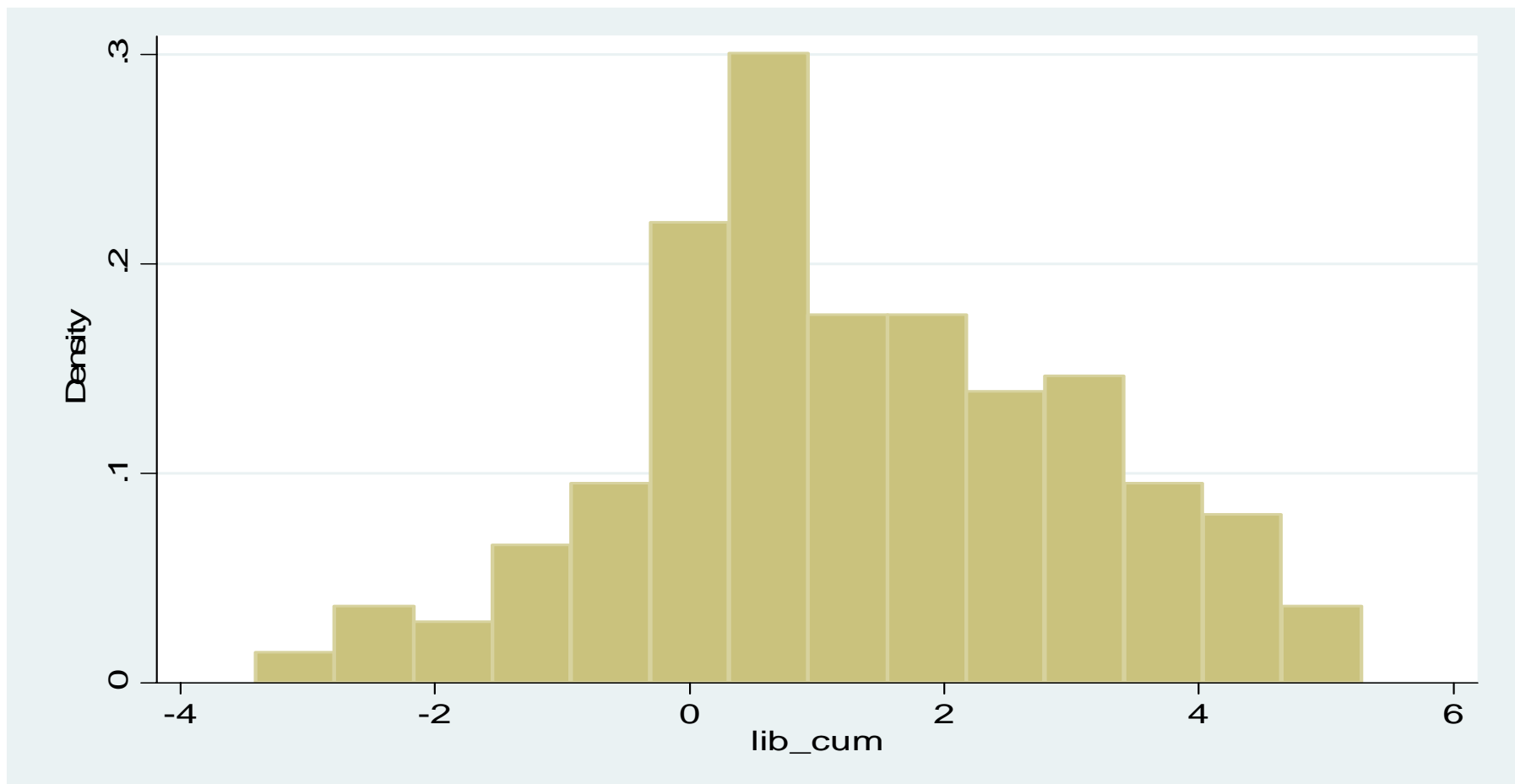
Figure 3. Histogram of the t-statistics of coefficients of cumulative effect of structural reforms on economic growth (221 coefficients from papers listed in Appendix 1)
