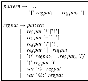
Figure 1. Regular expression pattern syntax
