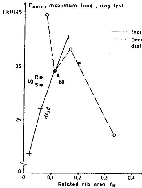
Figure 7: Load at ultimate bond resistance versus related rib area for the bars in SERIES 1, 2 and 3.
