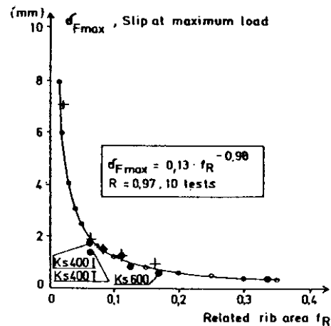
Figure 8: Slip at maximum load versus related rib area for the bars in SERIES 1, 2, and 3.
