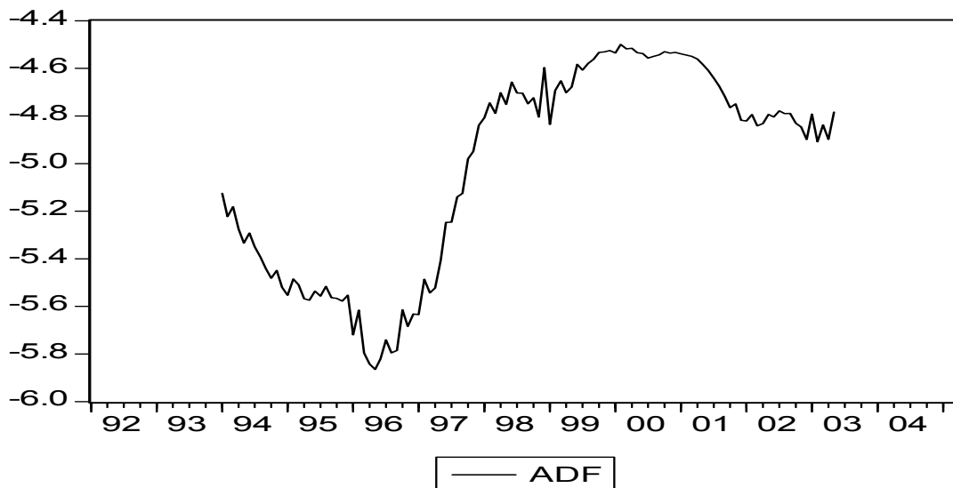
Figure 3: Recursively estimated Gregory – Hansen ADF statistics
