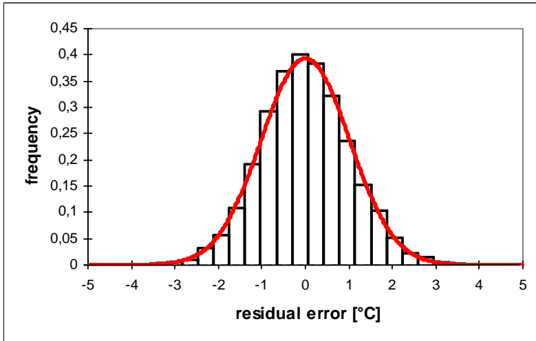
Figure 3: frequency distribution of the residual error
