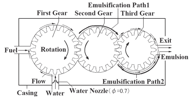
Fig.1 The scheme of top view of mechanical emulsifier (3-gears type) in this study.
