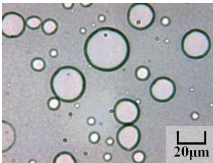
Fig.8 Microscopic photograph of water particles in the emulsified gas oil (Water: 9 vol.% for Fuel, 800 rpm).
