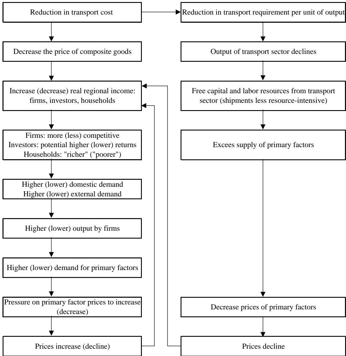
Figure 5. Causal Relationships in the Simulation
