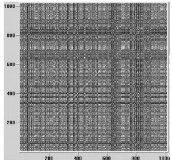
Fig.9: recurrence plot of "tent map" residuals
