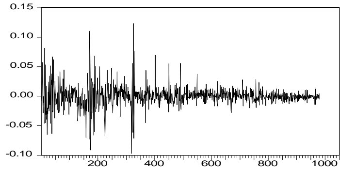
Fig. 13 industrial production residuals
