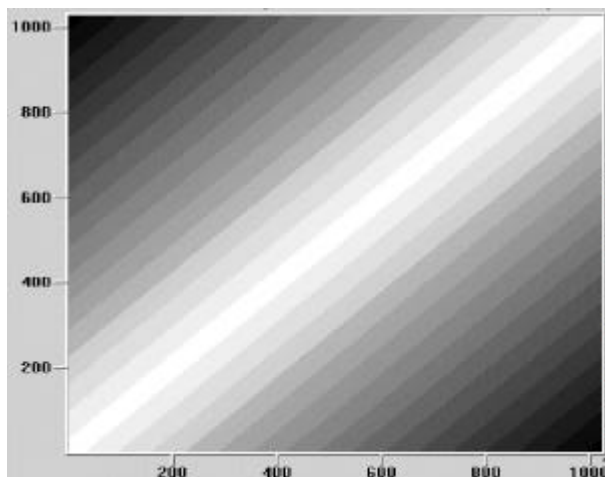
Fig.4: recurrence plot of a linear trend
