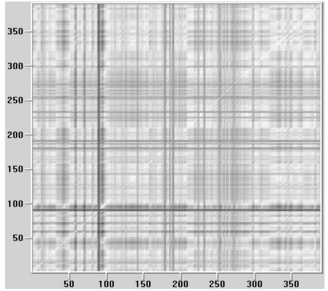
Fig. 18: HITEK production, recurrence plot
