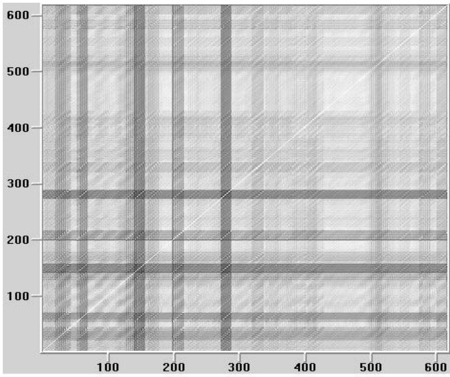
Fig. 15: Transportation equipment production, recurrence plot
