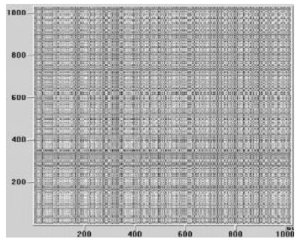
Fig.5: recurrence plot of i.i.d residuals
