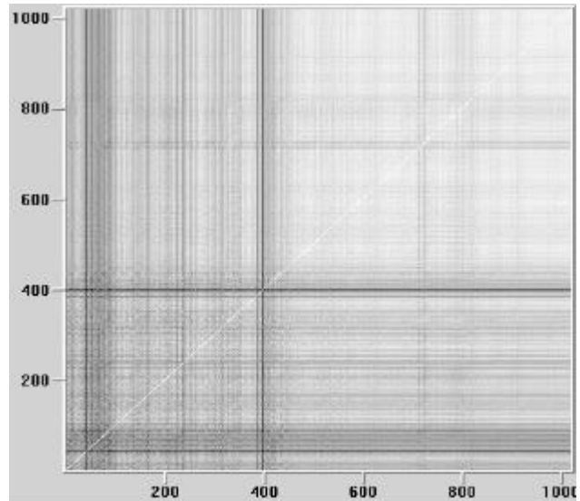
Fig. 21: consumer price index, recurrence plot
