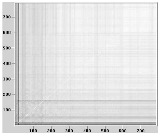
Fig. 18: HITEK production, recurrence plot
