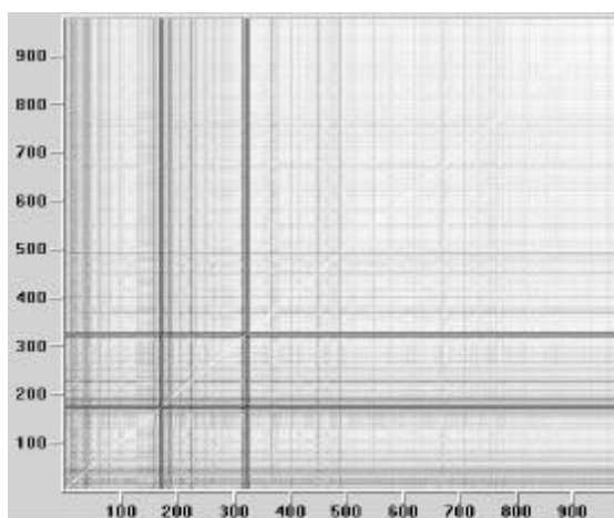
Fig.14: recurrence plot of residuals for industrial
