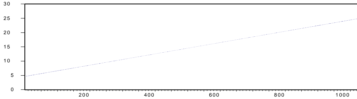
Fig.1: trend stationary growth
