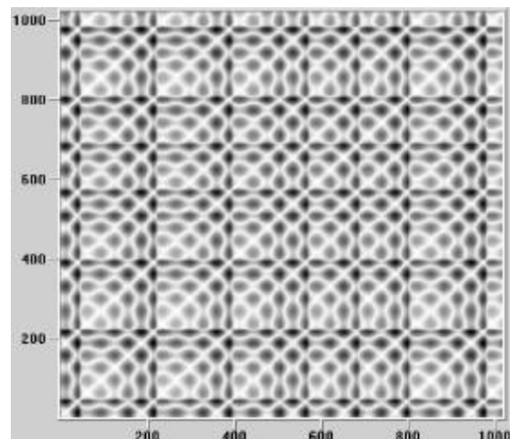
Fig.10: recurrence plot of "rossler" residuals
