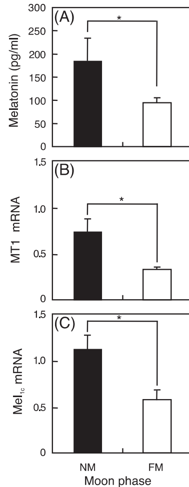
Fig. 2. Comparisons of melatonin concentration in the plasma (A), melatonin receptor, (MT1) gene expression in the pineal organ (B), and melatonin receptor (Mel 1c ) gene expression in the pineal organ (C) of the goldlined spinefoot between the new moon (NM) and full moon (FM). The plasma sample and the pineal organ were taken from fish at midnight during the new moon (■) and full moon (□). Melatonin levels in the plasma were measured by time-resolved immunofluoroassay. Expressions of MT1 and Mel 1c mRNA in the pineal gland were determined by quantitative real-time PCR and normalized by the amount of \beta -actin mRNA. Values are means \pm SEM. Asterisk indicates a significant difference ( p < 0.05 ) between the new moon and full moon. Modified from Ikegami et al. (2014).
