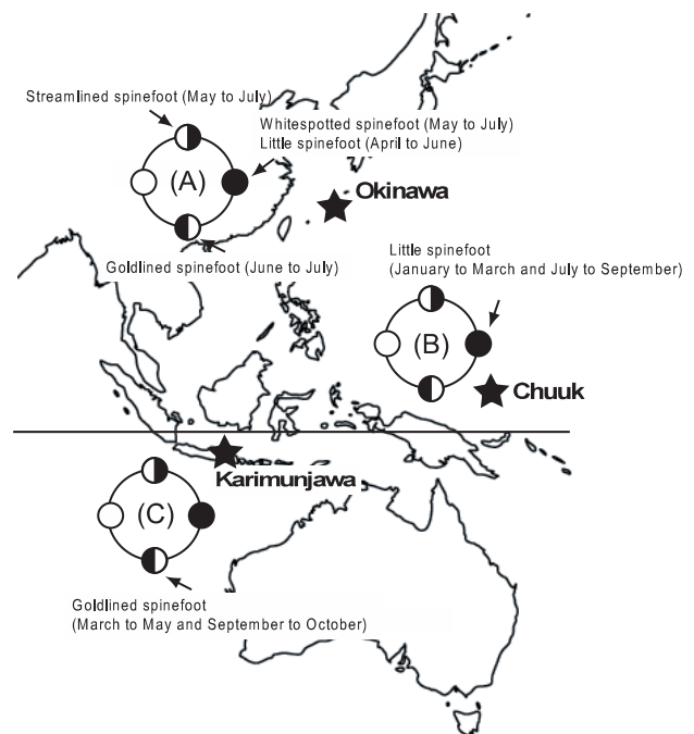
Fig.1. Geographical comparisons of annual reproductive cycle and spawning rhythmicity in spinefoot species in Indo-Pacific region. Stars indicate sampling sites; (A) Okinawa (Japan), (B) Chuuk (Micronesia), (C) Karimunjawa, Indonesia). Circles show lunar phase. ○; full moon, ◐; last quarter moon, ◑; new moon, ●; first quarter moon. Spawning lunar phase in each place is indicated by arrows.
