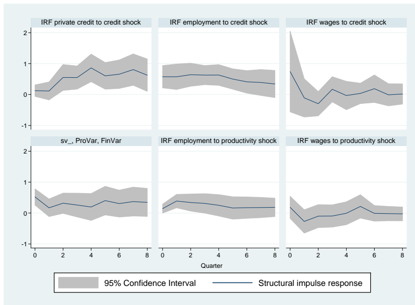
Figure 9: Four variables (exactly identified) VAR: TFP, private credit, employment and wages.
