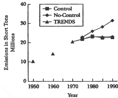
Figure 2. Comparison of control, no-control, and trends NO x emission estimates, 1950–1990
