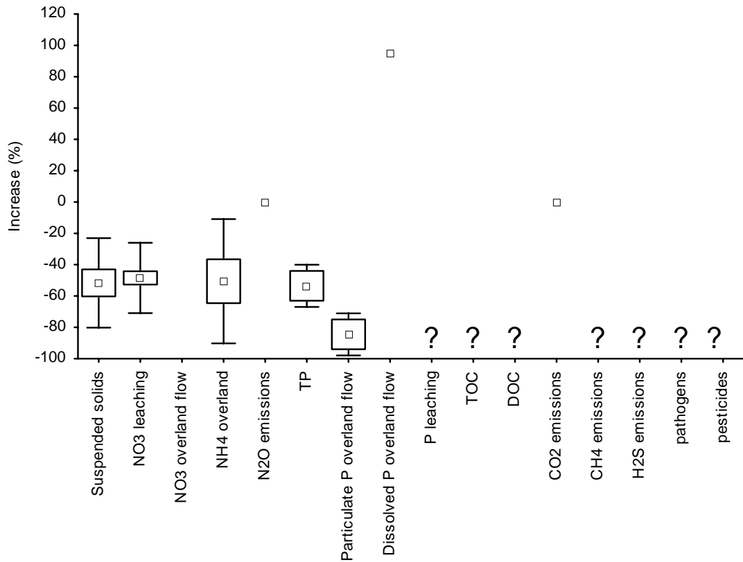
Figure 1. Percent reduction (-) or increase (+) from cover crops when compared to control plots in: suspended solids, NO 3 leaching losses, NO 3 losses in overland flow, NH 4 losses in overland flow, N 2 O emissions, total P losses on overland flow, dissolved P losses in overland flow, P leaching, total organic carbon losses in overland flow, dissolved organic carbon losses in overland flow, CO 2 emissions, CH 4 emissions, H 2 S emissions, pathogens in overland flow and overland flow pesticide losses. Data for suspended solids was taken from 81 and 88 (n=12). NO 3 leaching losses were taken from 7, 12, 14, 34, 43, 99, 104, 105, 114, 117, 119, 156, 157, 181, 184 (n=38), NH 4 in loads in overland flow from 152 (n=8), N 2 O emissions from 193 (n=1), total P losses in overland flow data were from 167, 187(n=2), particulate P losses from 187, 167 (n=2) and dissolved P losses from 187(n=1). CO 2 emissions were taken from 193 (n=1). □ Mean, □ Mean ± Standard error, | Mean ± standard deviation, ↑ indicates trend reported in literature, ? indicates no information. No error bars indicates insufficient data.
