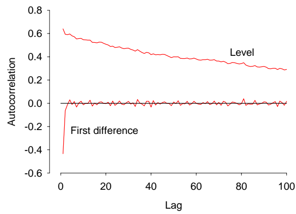
Figure 5: Autocorrelation functions from lag one for the Ericsson series and its first differences.
