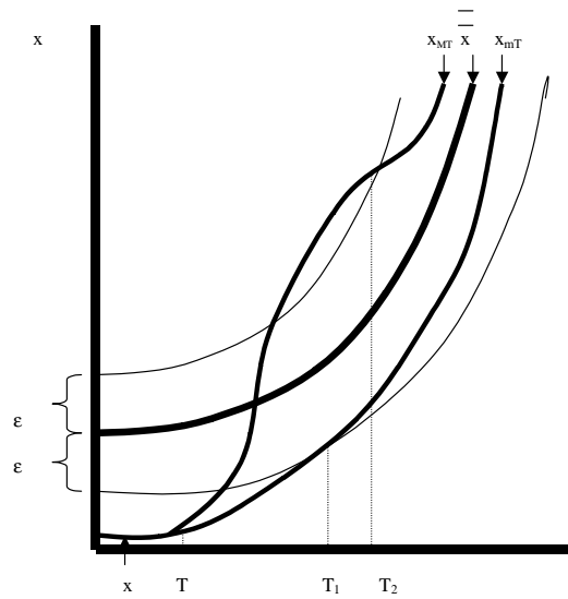
Figure 1. Illustration of lemmas 6 and 7
