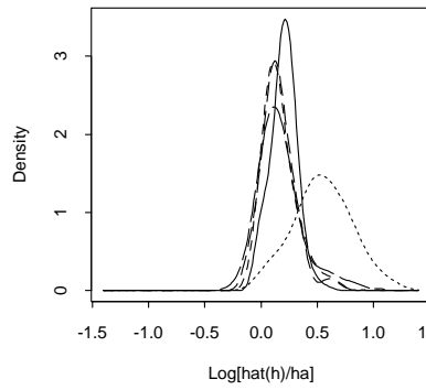
Figure 3g: m=1, \phi_1=-0.3 , all delta's
