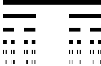
Figure 1: Middle-third Cantor set
