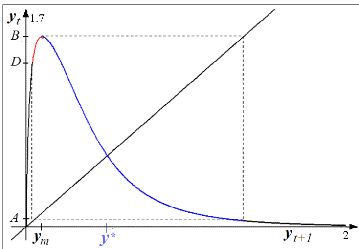
Figure 5: Graph of the one-dimensional function \chi at l^* = 2 , \alpha_1 = 0.5 and \alpha_2 = 6 . \chi_L is the branch on the left of the critical point y_m with inverse \chi_L^{-1} , \chi_R is the branch on the right of y_m with inverse \chi_R^{-1} . The interval of interest is I = [A, B] = [A, D] \cup [D, B] , where B = \chi(y_m) , A = \chi^2(y_m) , D = \chi^3(y_m) .
