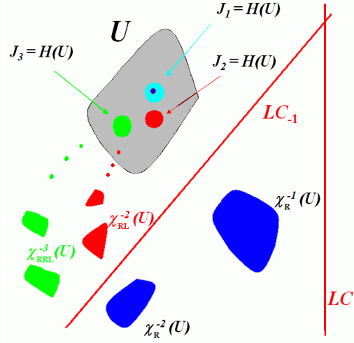
Figure 12: Qualitative description of the construction of the different sets J_1 , J_2 and J_3 belonging to U , involved in the IFS similar to the "chaos game" associated with the two-dimensional model. X^* \in J_1 .
