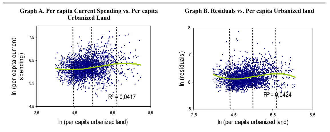
Figure 2. Scatter diagrams
