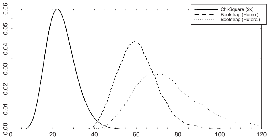
Figure 5. Sunspot series asymptotic and bootstrap distributions of F_{13} .
