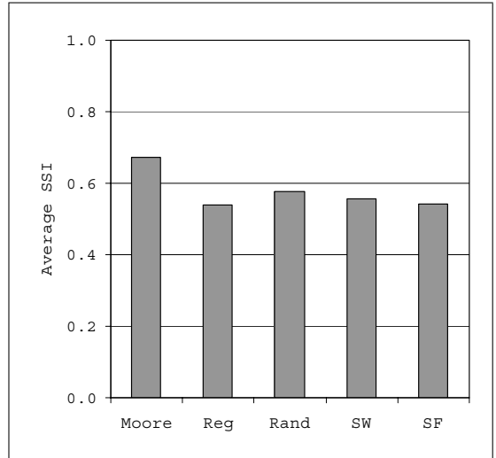
Figure 5: Average Spectral Segregation Index (SSI) v. Network Classes. Average Degree d = 8 . Parameters: M = 100 , \theta = 0.3 . MC Sample Size = 1000.
