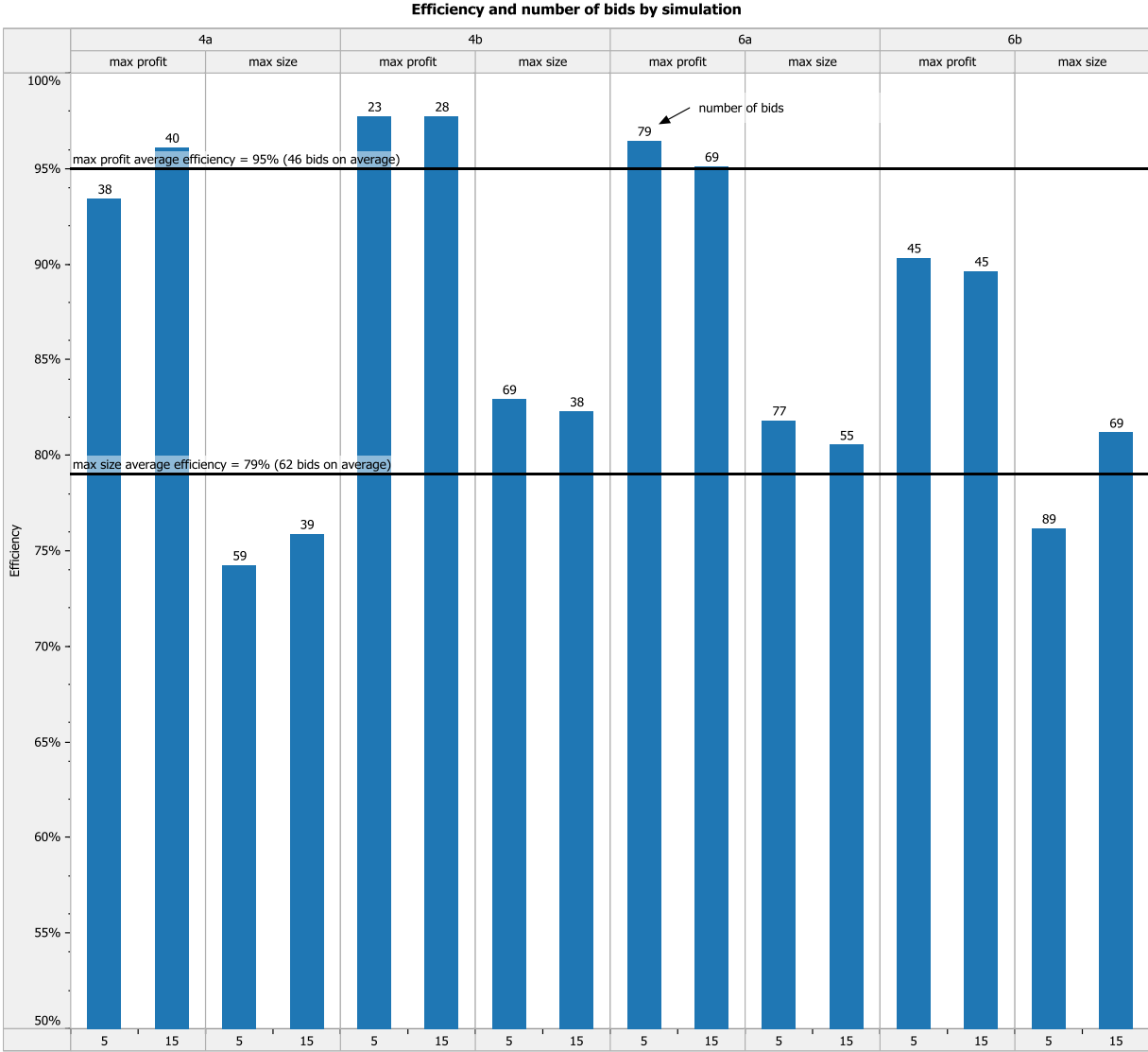
Figure 8. Revealed preference rule yields higher efficiency and fewer bids in the clock stage
