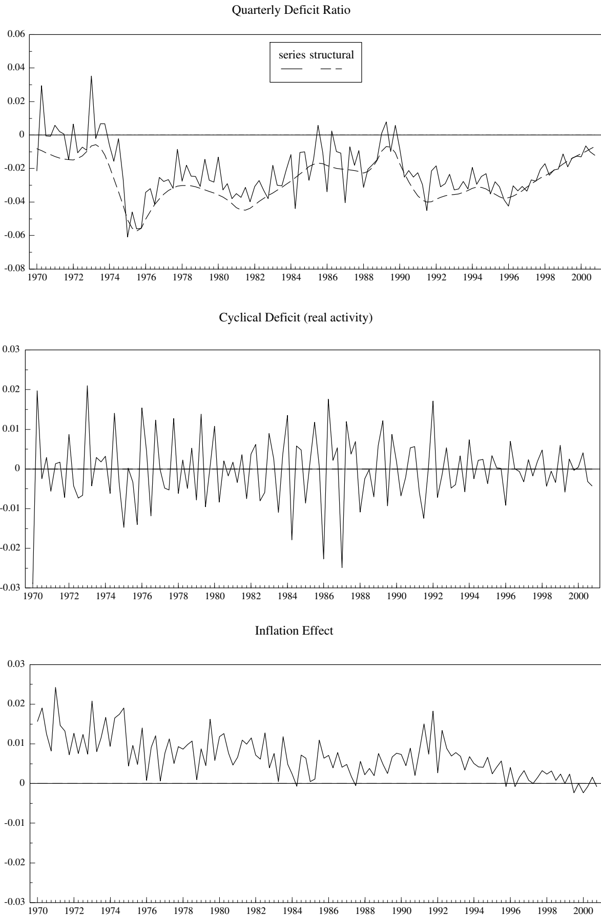
Figure 2: Quarterly Deficit Series Decomposition. Germany. Model 2.
