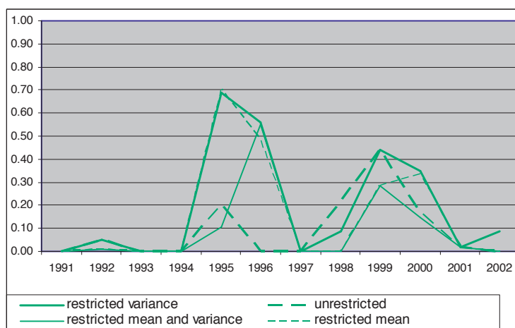
(4.b) MMM estimates of DNWR
