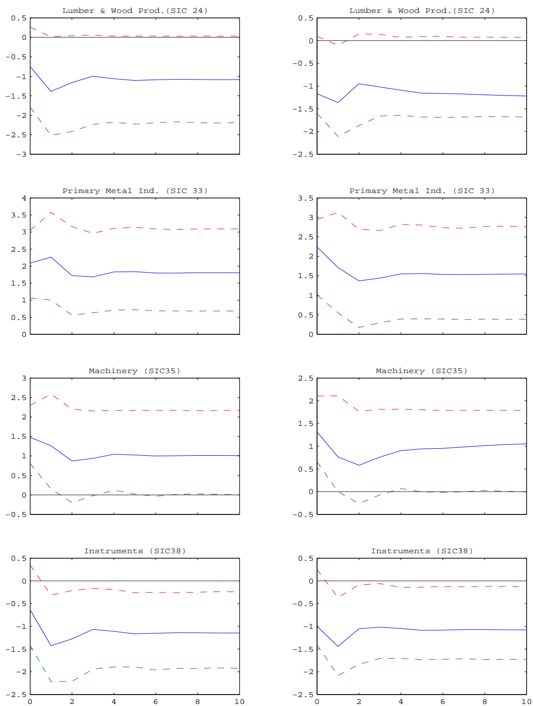
Figure 5: Response functions of the labor productivity to a nontechnology shock, under the Galí assumption, for r = 4 (left-side) and r = 7 (right-side).
