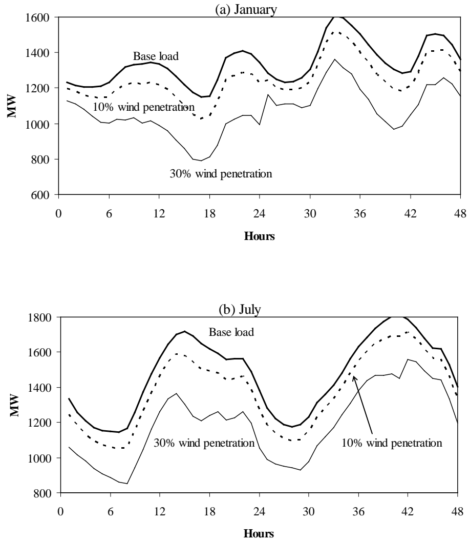
Figure 3: Load to be met by traditional generators for the first two days (48 hours) in (a) January and (b) July (adjusted ERCOT load data). Demand after non-dispatchable wind power has been subtracted has greater variability than the non-wind load, although the adjusted series still track the morning (0600-1200) and evening (1800-2300) peaks quite well. If a longer profile were chosen, the volatility would be even sharper.
