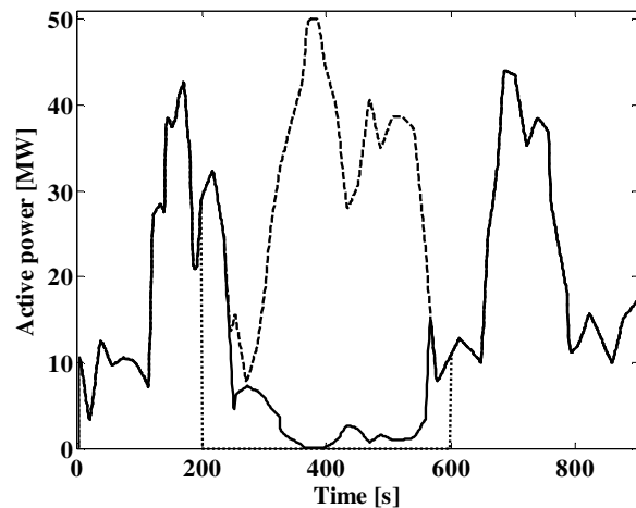
Figure 11: Power of the WF2. Dash-dotted line: Without congestion management. Full line: With real-time supervisor. Dotted line: With actual method.
