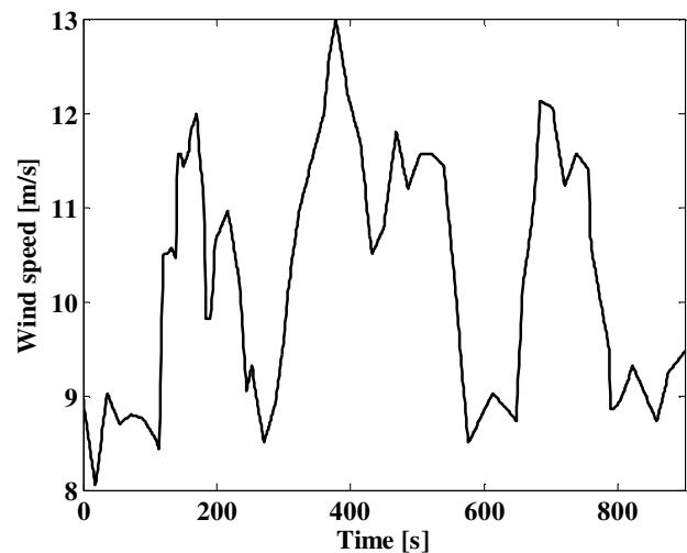
Figure 9: Wind speed.
