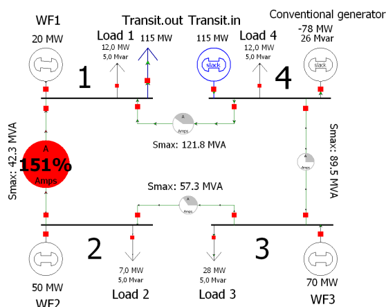
Figure 1: Test system.
