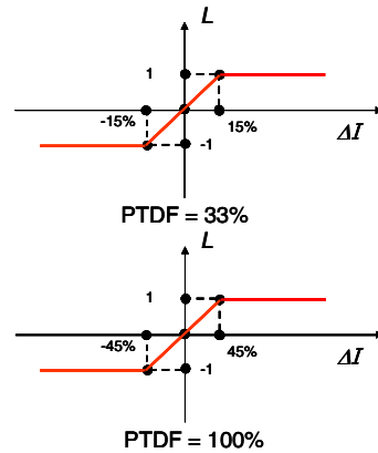
Figure 6: Adjustment of the signal L based on the PTDF of the units realizing the re-dispatching and the amount of overload.
