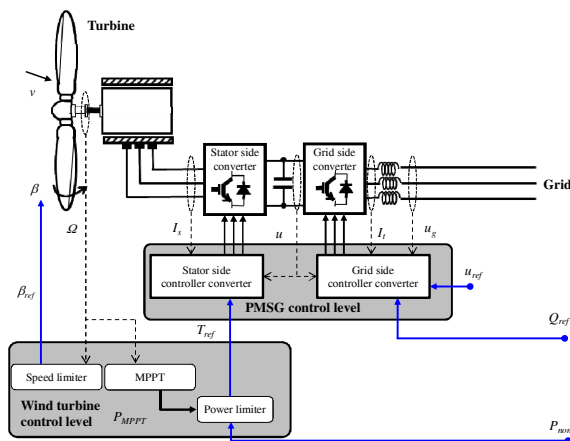
Figure 2: Wind turbine model.
